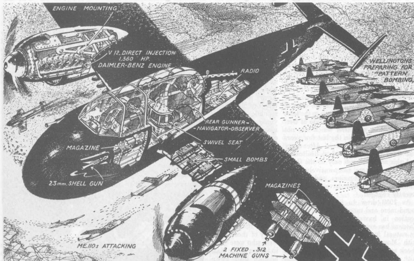
The Messerschmitt ME110, shown here in sectioned diagram, is a new design of fighter aircraft that was used by the Nazis in the Polish campaign, and machines of this type have now reinforced the defence forces on the north-west coast of Germany. Coming into the twin-engine two-seater class, it is exceptionally fast and well armed. The drawing indicates the position of the six forward guns; there may be also a rear gun for the observer, and this is shown. In the great air battle near Heligoland on December 18, an ME110 was employed as an interceptor fighter against the R.A.F. "Wellingtons," but its value for bomber escort, ground attack, or reconnaissance has not been overlooked.
