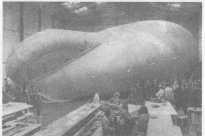
The work of manufacturing barrage balloons needs the finest workmanship and special training is given to the "hands." Left, girls are attending a course in which a small model of a balloon is being used to show the general construction. Above, air is being pumped into the stabilizer during a final test of a balloon.
