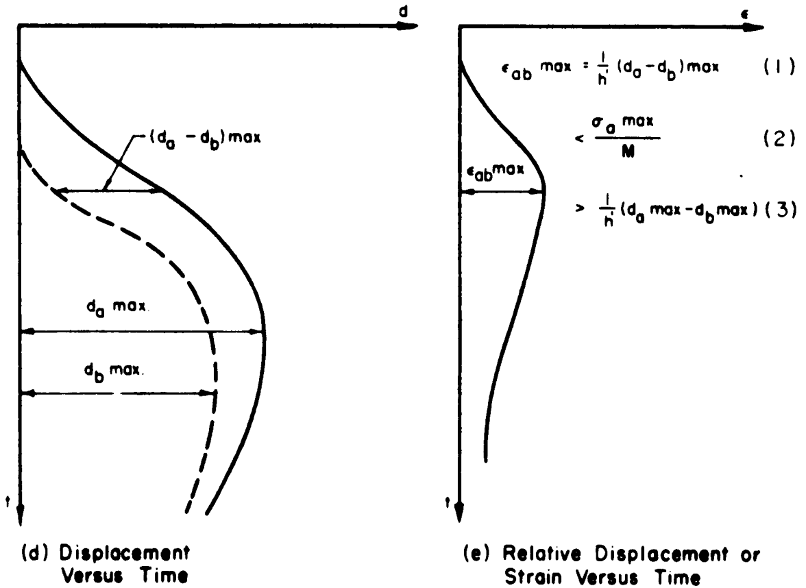
FIG. 4-10 EVALUATION OF PEAK RELATIVE DISPLACEMENT
