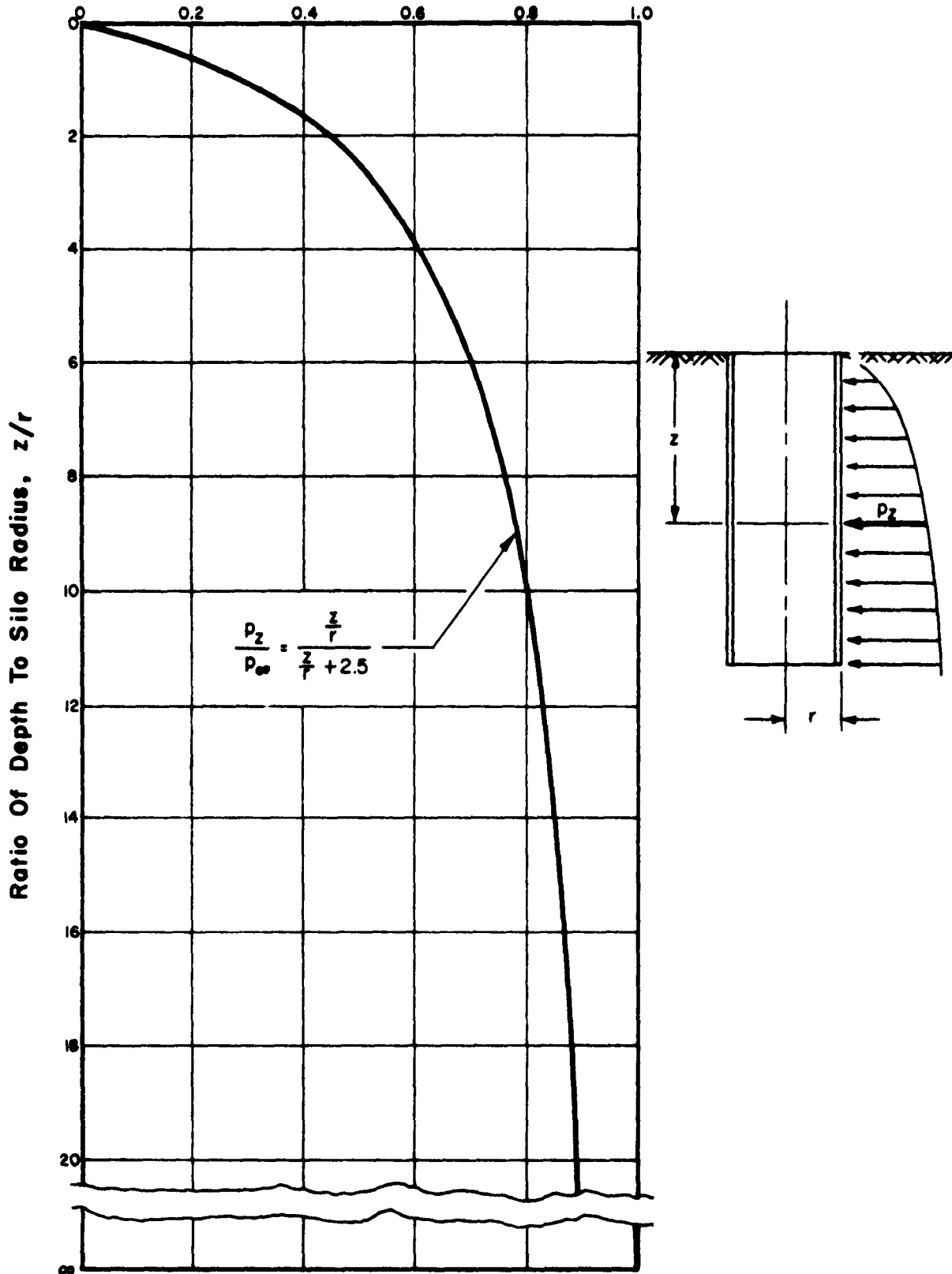
FIG. 5-17 HORIZONTAL DEAD LOAD PRESSURE DISTRIBUTION AGAINST SILO
