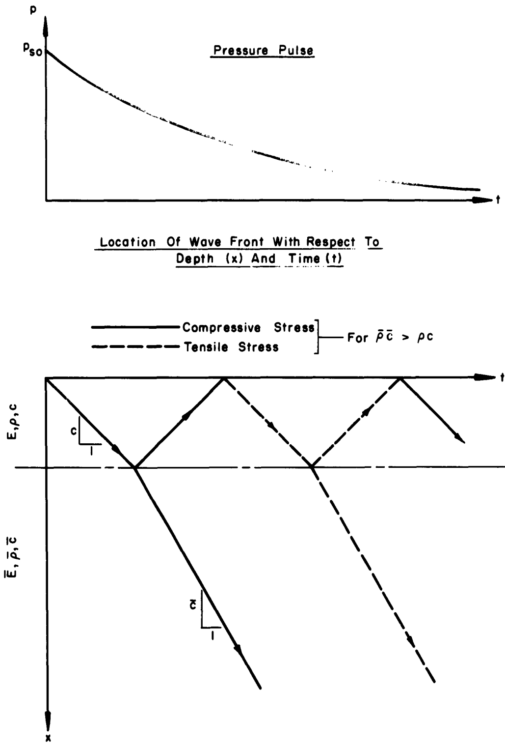
FIG. C-3 ONE-DIMENSIONAL WAVE IN A LAYERED MEDIUM
