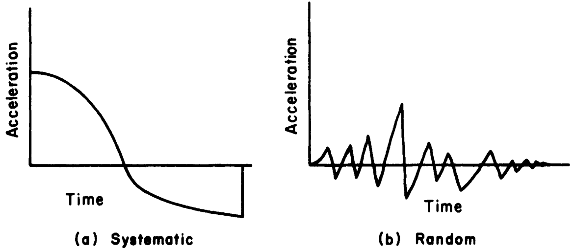
FIG. 10-2 COMPONENTS OF GROUND MOTION
