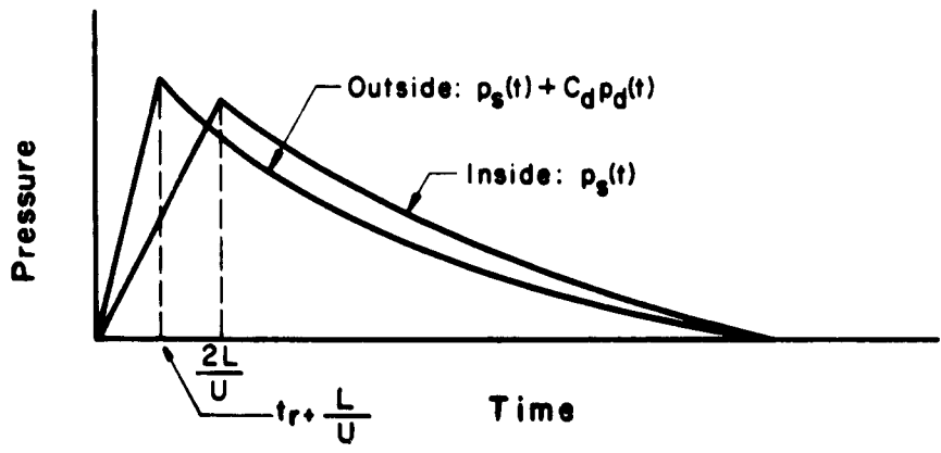
(c) Roof Loading
