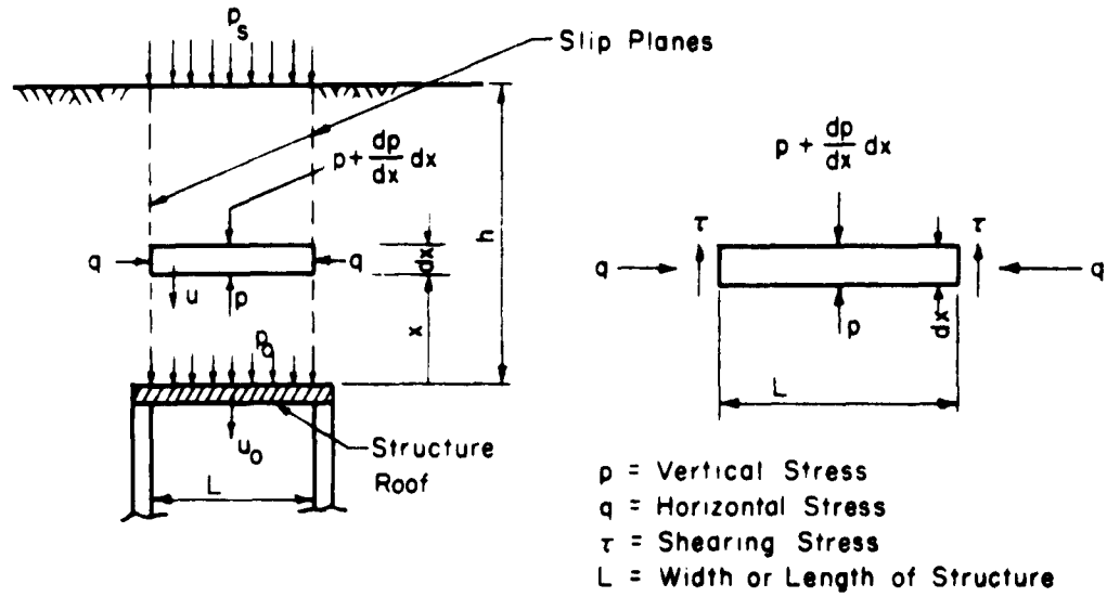
FIG. 5-9 FORCE FIELD ASSUMED FOR UNDERGROUND STRUCTURE
