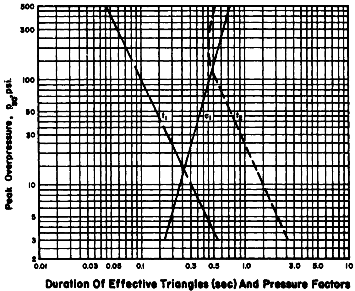
FIG. 3-8 TWO-TRIANGLE REPRESENTATION FOR OVERPRESSURE—IMT SURFACE BURST
