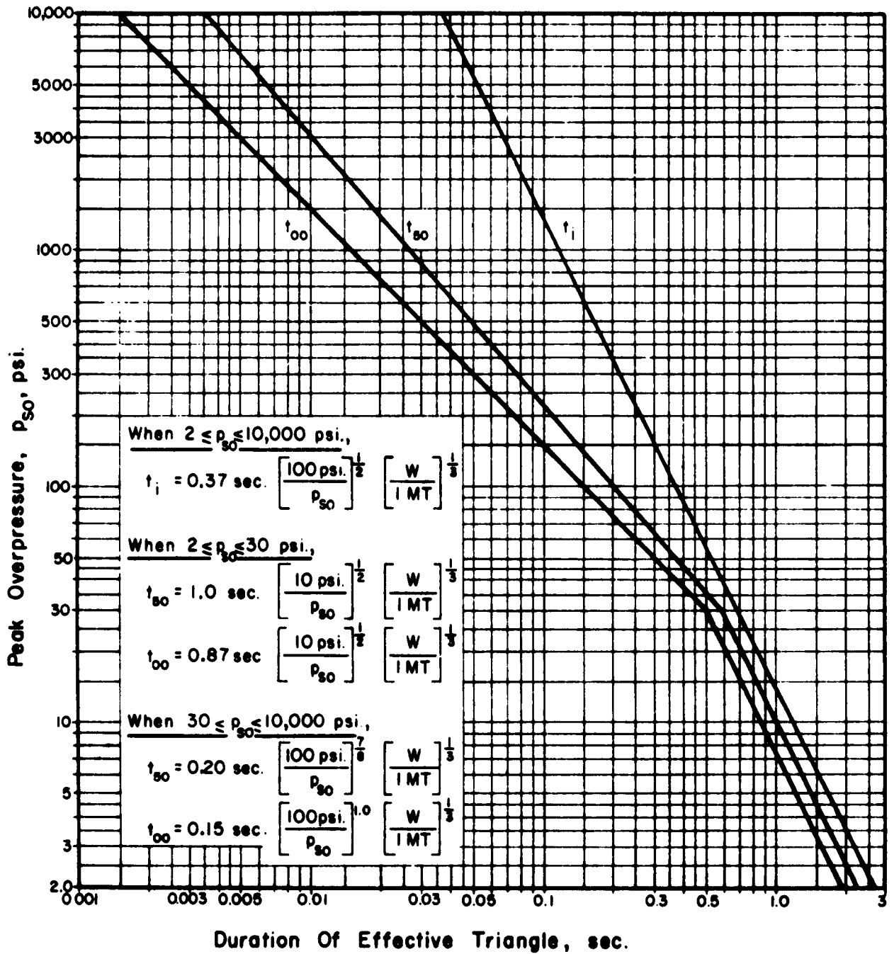
FIG. 3-7 DURATION OF EFFECTIVE TRIANGLES FOR REPRESENTATION OF OVERPRESSURE-TIME CURVES — I MT SURFACE BURST
