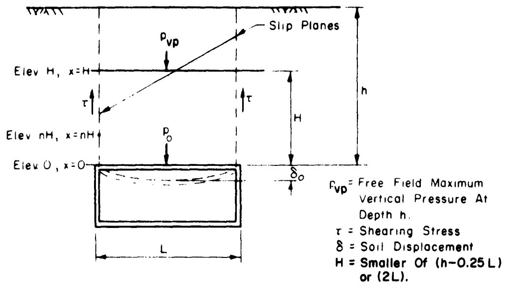
FIG. 5-13 CROSS-SECTION OF UNDERGROUND STRUCTURE
