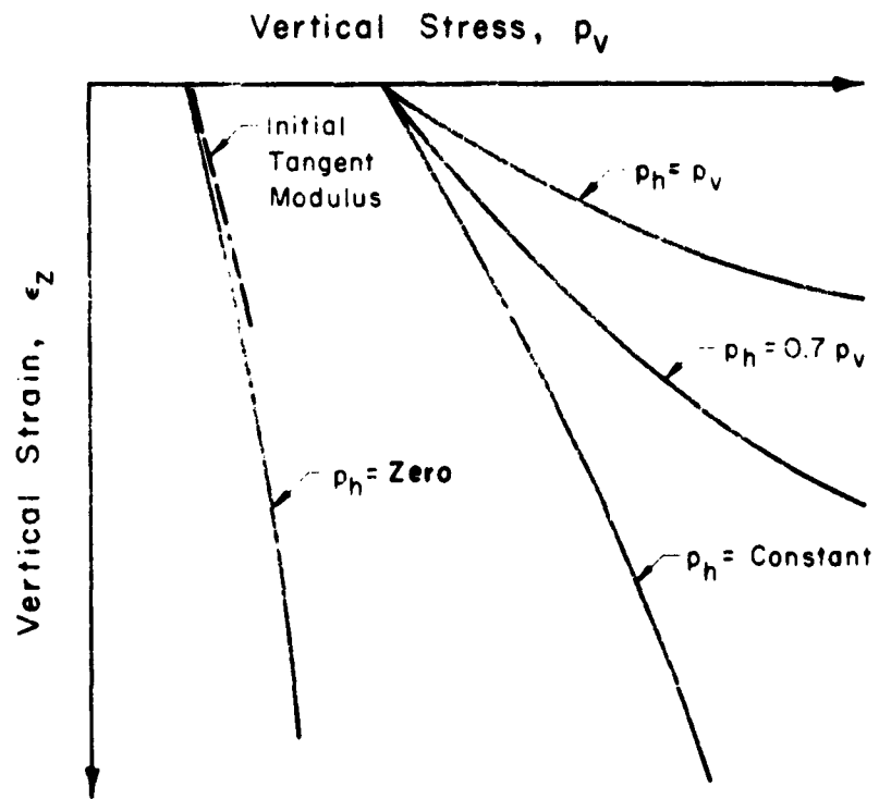
FIG. 4-5 TYPICAL SOIL CONSOLIDATION CURVES.
