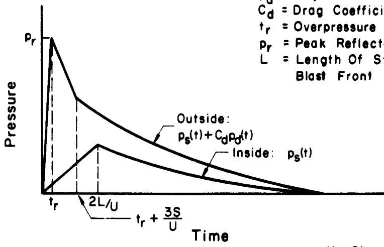
(a) Windward Wall Loading
