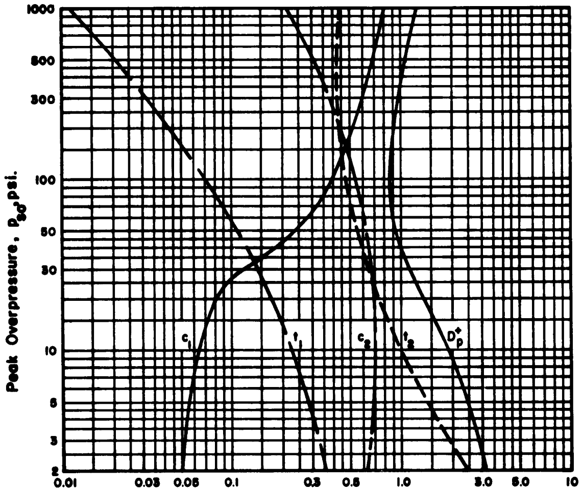
Duration Of Effective Triangles (sec.) And Pressure Factors
