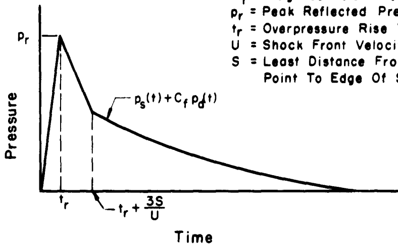
(a) Windward Wall Loading
