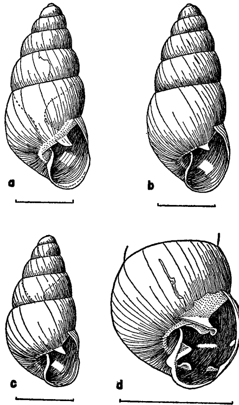
FIGURE 8.— a , Tubuaia voyana matonaensis , Rurutu, adult (holotype). b , T. v. turivaoensis , Raivavae, adult (holotype). c , d , T. v. vaiaumanae , Raivavae: c , adult (holotype); d , metaneanic, oblique apertural view illustrating strongly sinuous parietal lamella and biplicate palatal wall (faint subcolumellar fold is shown).
