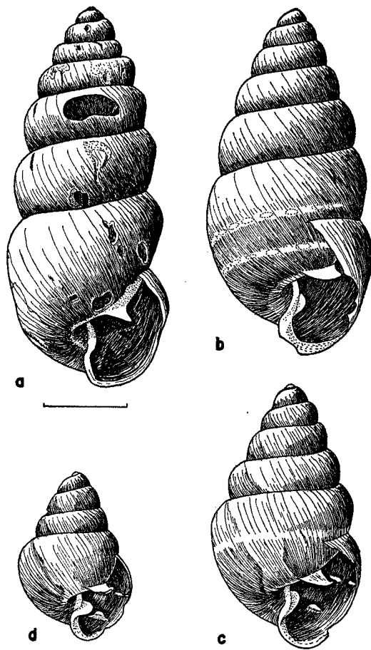
FIGURE 4.— Tubuaia fosbergi , Pitcairn: a, adult (holotype); b, paraneanic, oblique view; c, metaneanic, frontal view; d, meta-ananeanic, frontal view.
