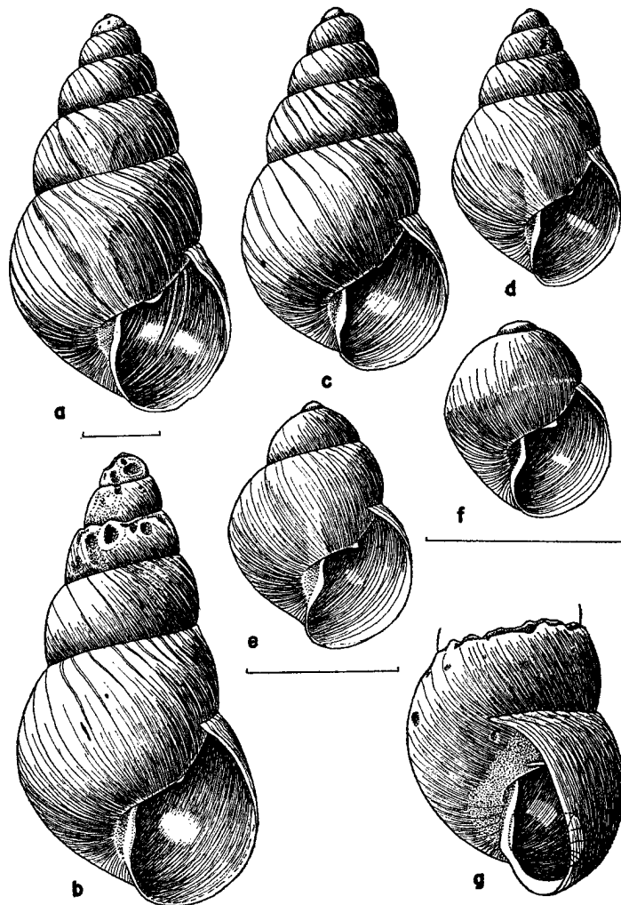
FIGURE 14.— Tubuacia saintjohni , Raivavae: a, adult (holotype); b, large adult; c, paraneanic; d, metaneanic; e, ananeanic; f, embryo; g, adult, oblique view, with vestigial columellar lamella.
