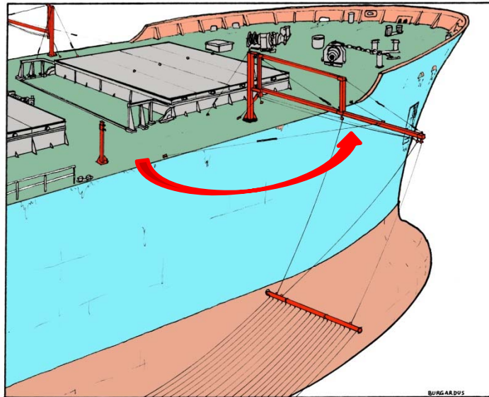
Swivelboom
