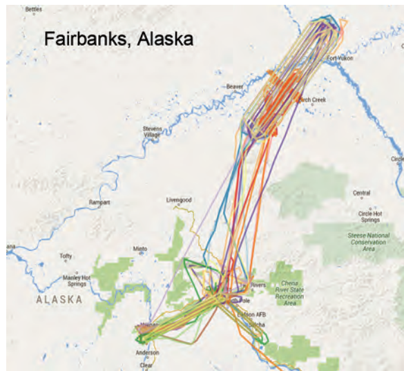
FIGURE 17 2015 AirSWOT flights
