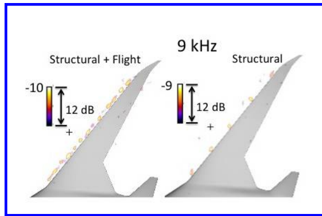
Figure 18: Krueger brackets are the dominate noise source at 9 kHz. 13
