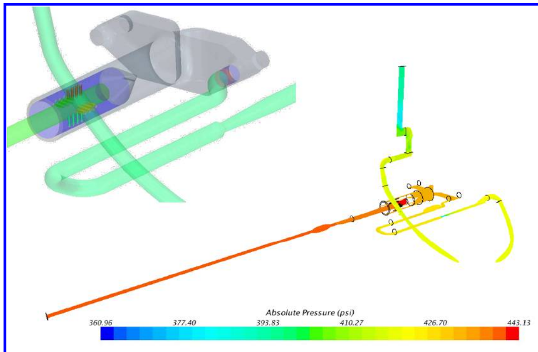
Figure 25: Geometry of the flow through balance as tested in the ARC UPWT 9- by 7-foot Supersonic test section.
