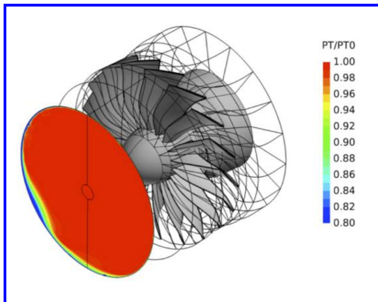
Figure 27: Sample CFD++ solution of inlet distortion mapped to fan face. 3
