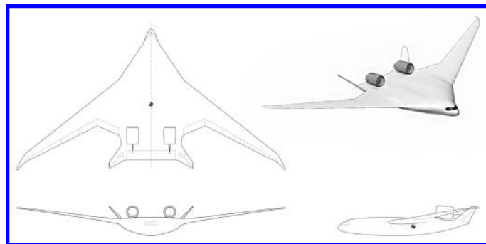
Figure 10: Three view of the ERA-0009GM
