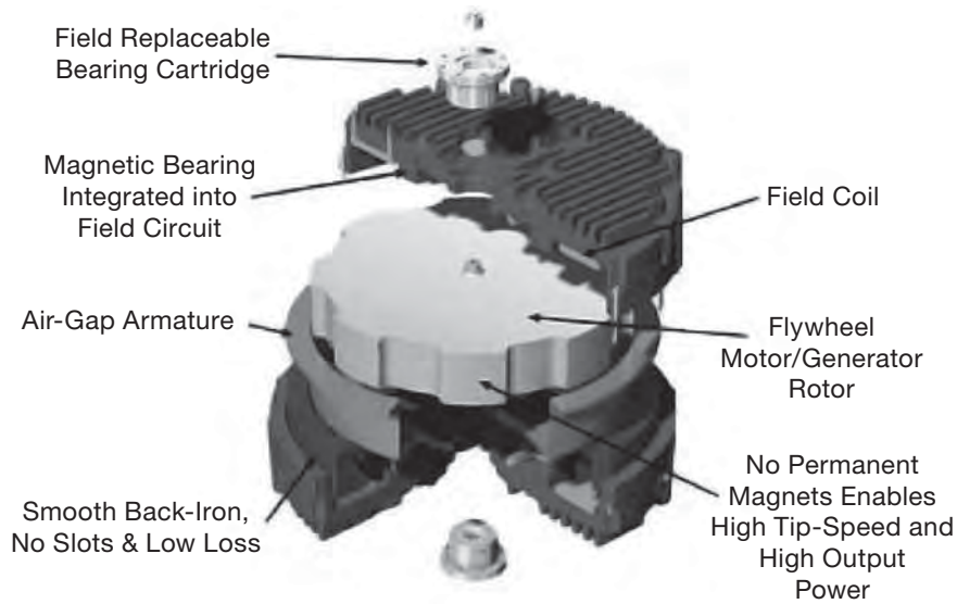
Figure 2-4 | Flywheel energy storage [act11]
