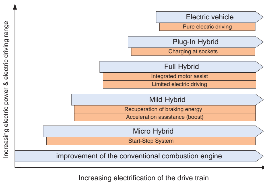
Figure 3-16 | Hybrid classes sorted by electrical power and functional range, against stage of development (Fraunhofer ISE)
