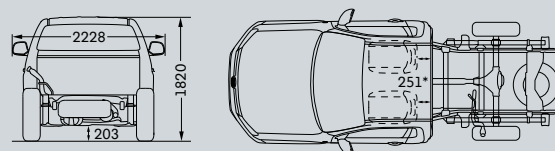
Amarok Single Cab Chassis
