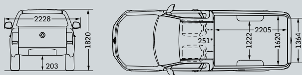
Amarok Single Cab
