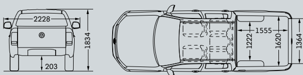
Amarok Dual Cab
