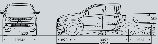
Amarok Dual Cab
