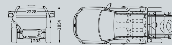
Amarok Dual Cab Chassis
