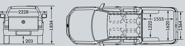
Amarok Dual Cab – Trendline, Highline and Ultimate
