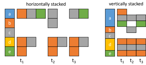
Figure 12: Two variants of list representations visually encoding a dynamic graph by color-coded targets of edges.
