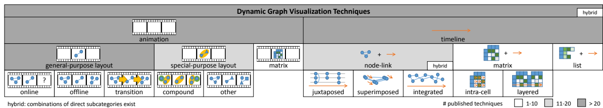
Figure 1: Illustrated hierarchical taxonomy of dynamic graph visualization techniques; the number of published techniques per taxonomic category is encoded in the brightness of the background (for details see Table 4 and Table 5).
