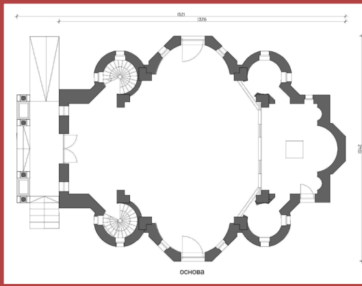
Основа – проект – црква Foundation – project – church
