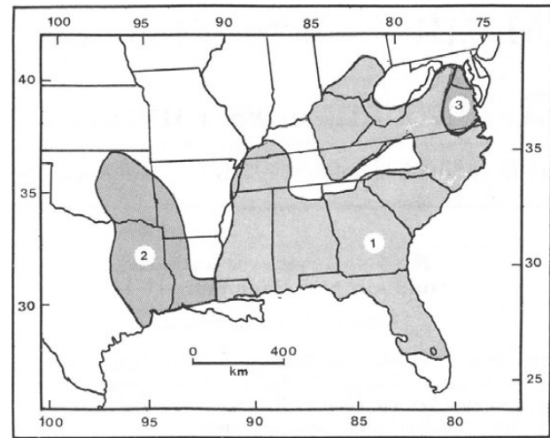
FIG. 3. Distribution of Reithrodontomys humulus in the United States (modified from Hall, 1981, with addition of peripheral trap records from >40 publications and personal correspondence): 1, R. h. humulus ; 2, R. h. merriami ; 3, R. h. virginianus .
