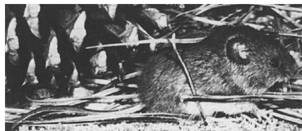
FIG. 1. Adult Reithrodontomys humulis . Photograph by R. W. Van Devender.
