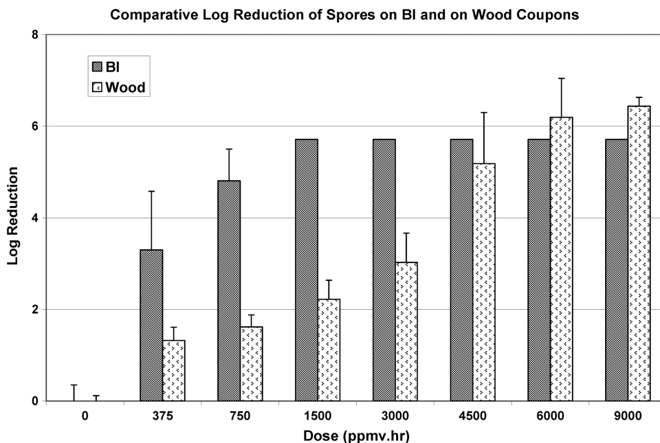
FIG. 4. Log reduction of viable spores on BIs and wood coupons with 500 ppmv of CSI CD gas.
