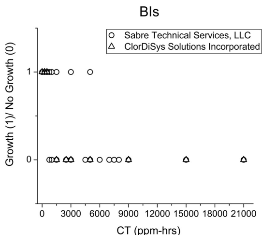
FIG. 3. Number of BIs testing positive (represented as 1) or negative (represented as 0) based on turbidity as a function of CD gas dose.
