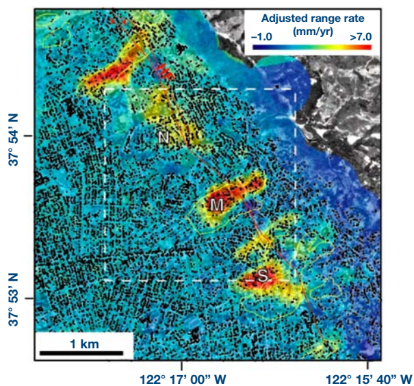
Potential landslides are readily identified in this interferogram of the Berkeley hills in California. Rain causes slipping of the hillsides.
