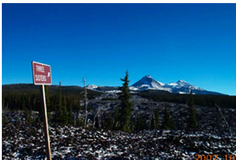
Figure 5. InSAR studies in the Cascade Ranges have found that observed uplift of 4 cm/yr is due to magma injection at a depth of 8 km. (Figures courtesy of W. Thatcher, USGS.)
