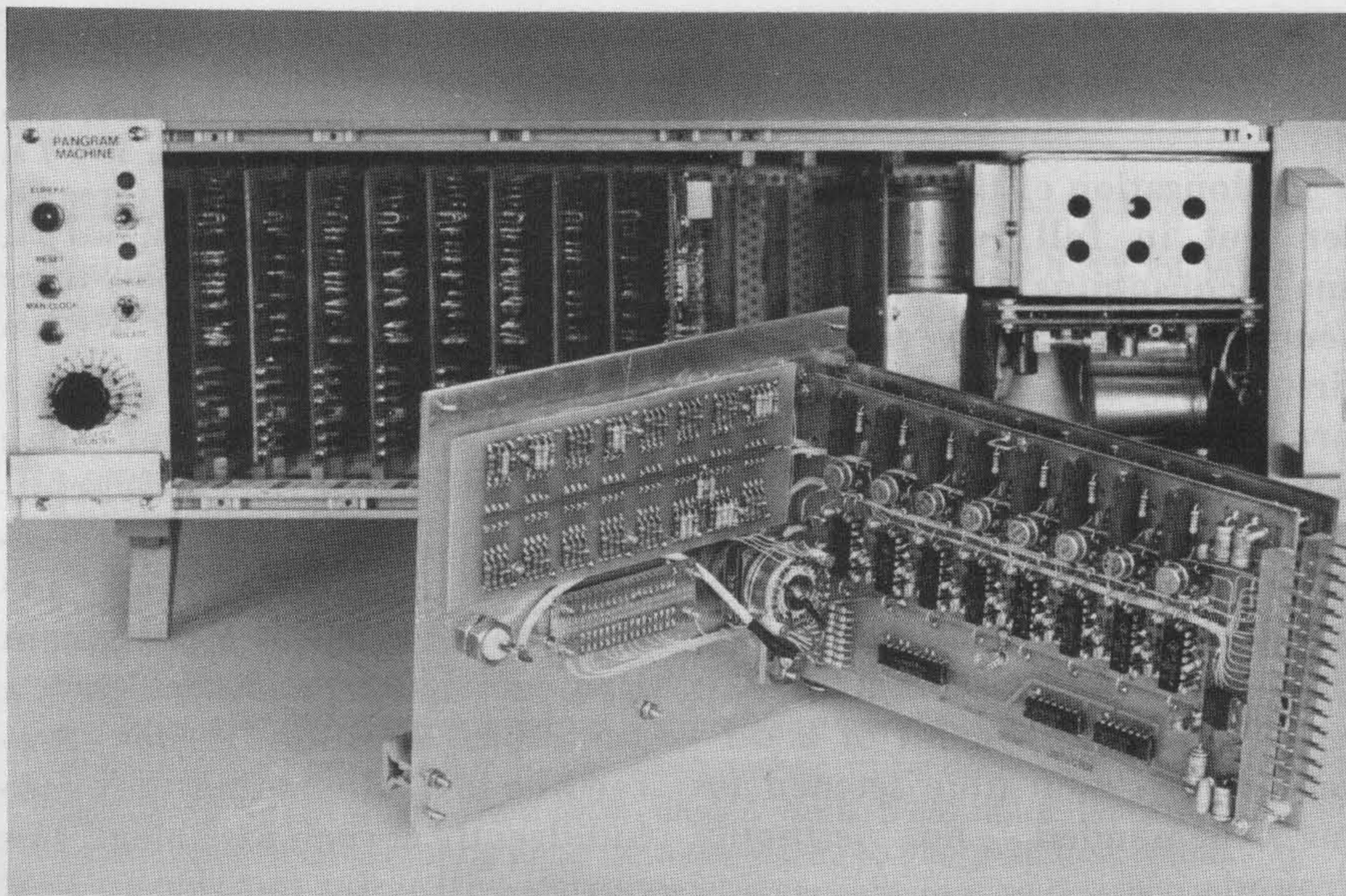
Two printed circuit cards behind the right-hand front panel carry the sixteen BALANCE-detectors. The circular metal cans are differential amplifiers, below which a line of eight integrated circuits form the ZERO? detectors. On the panel itself are the initial text-constant resistors selected by means of the PRESET LETTER WEIGHTS switches.
