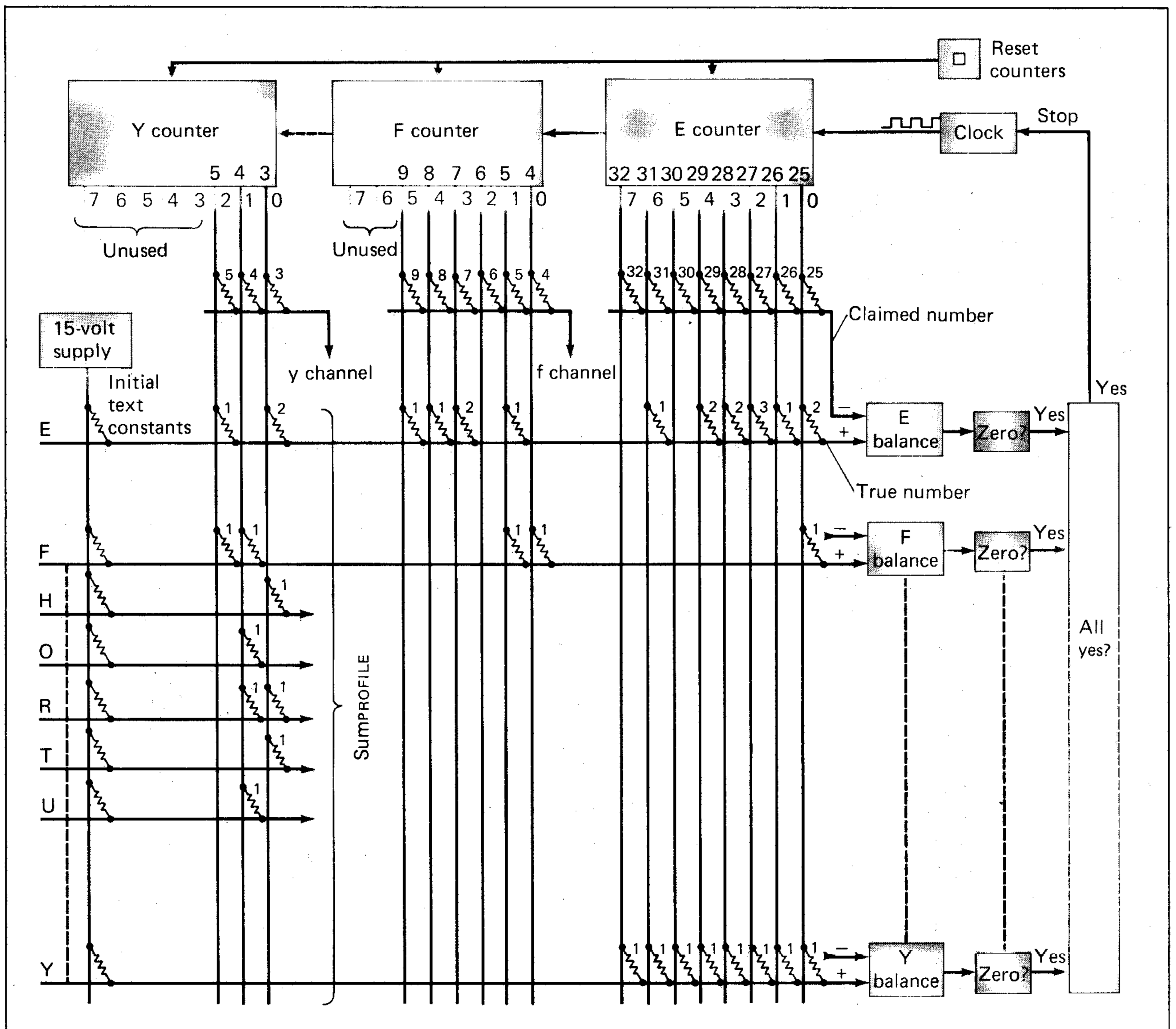
Figure 3. The design of the Pangram Machine.
