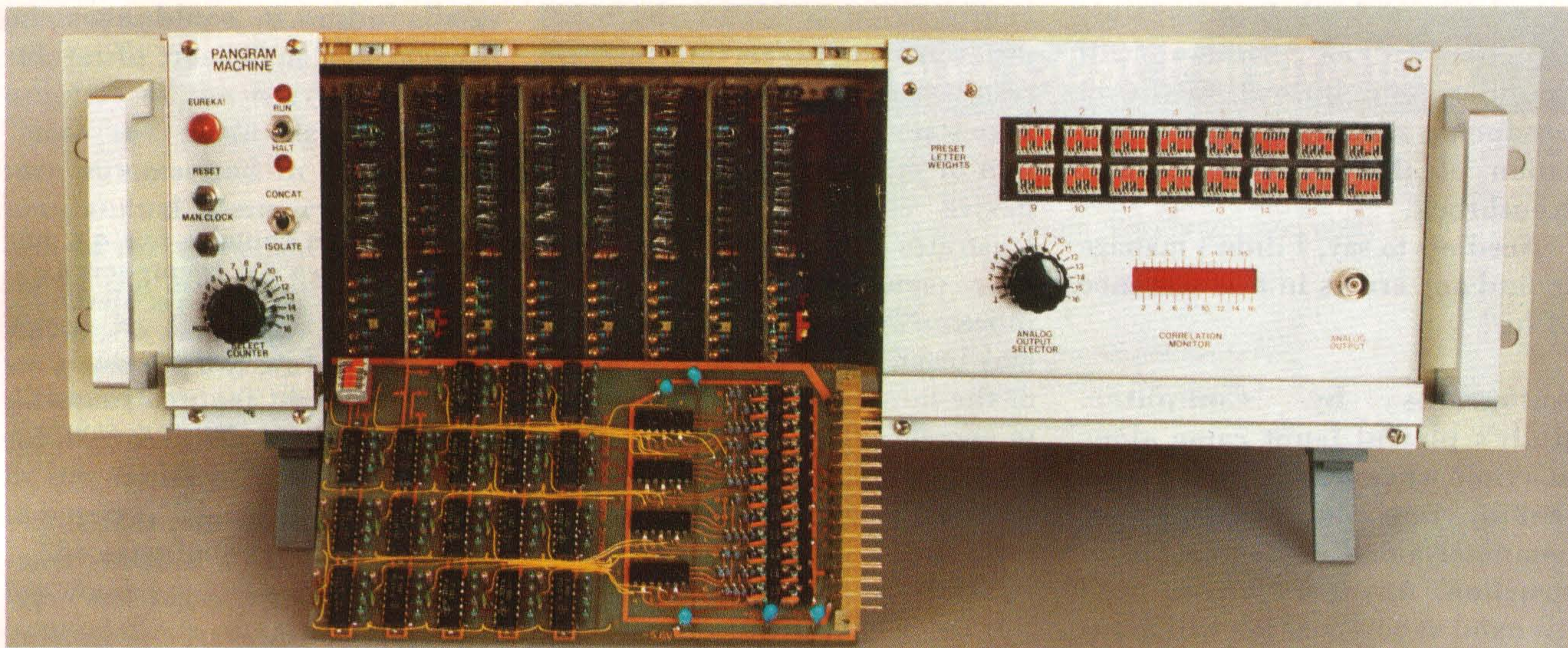
The automatic number-word selector board that transformed the original pangram machine into the Mark II version. On the left, 18 window-detector chips determine the number of g 's, l 's, x 's, and y 's. At right, 4 more integrated circuits and 24 transistors switch in the appropriate PROFILES on the resistor-bearing cards above.
