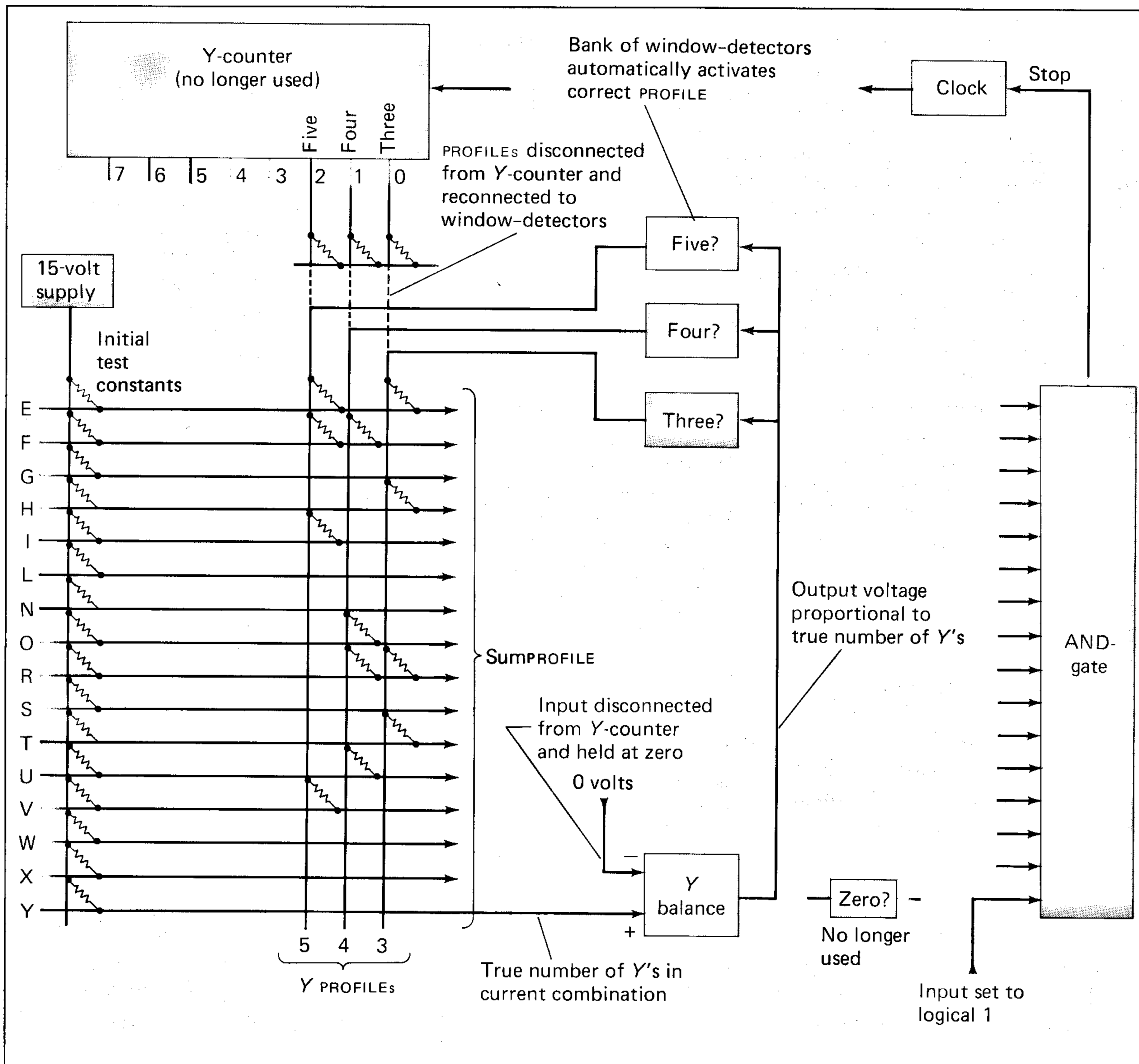
Figure 5. Example of automatic number-word selection applied to the letter y . A voltage proportional to the number of y 's occurring in the present combination is classified by a bank of three window-detectors, one of whose outputs will activate the appropriate PROFILE.
