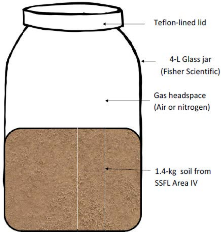
Figure 1: Glass jars for laboratory microcosms (not to scale)
