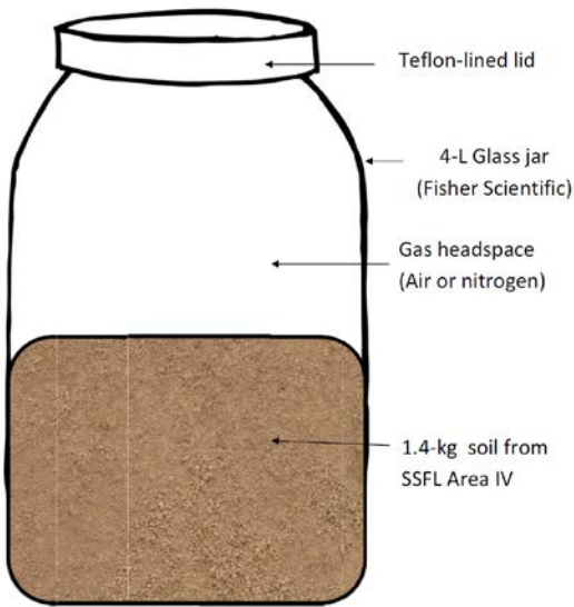
Figure 4-3 Bioremediation Treatability Soil Microcosms
