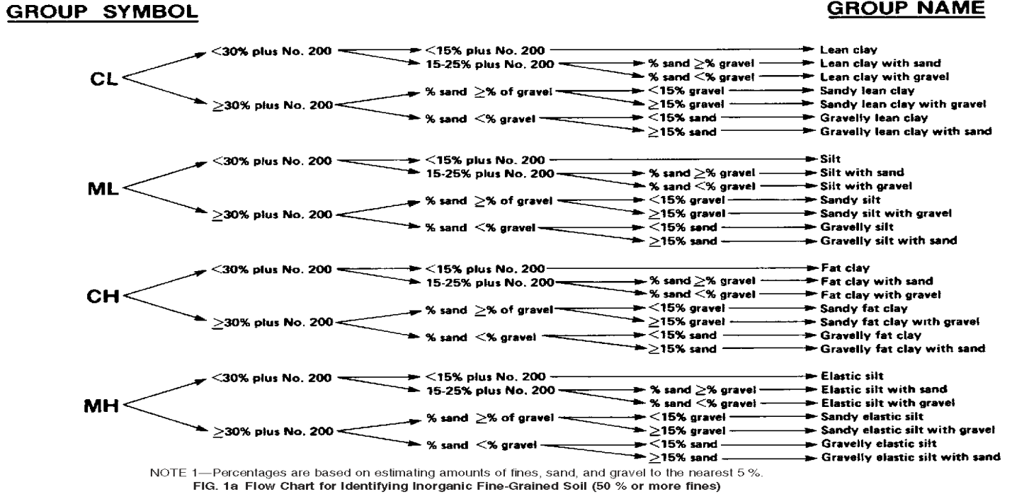
FIG. 1a Flow Chart for Identifying Inorganic Fine-Grained Soil (50 % or more fines)
