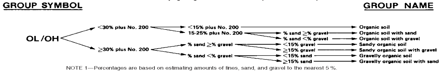
FIG. 1 b Flow Chart for Identifying Organic Fine-Grained Soil (50 % or more fines)
