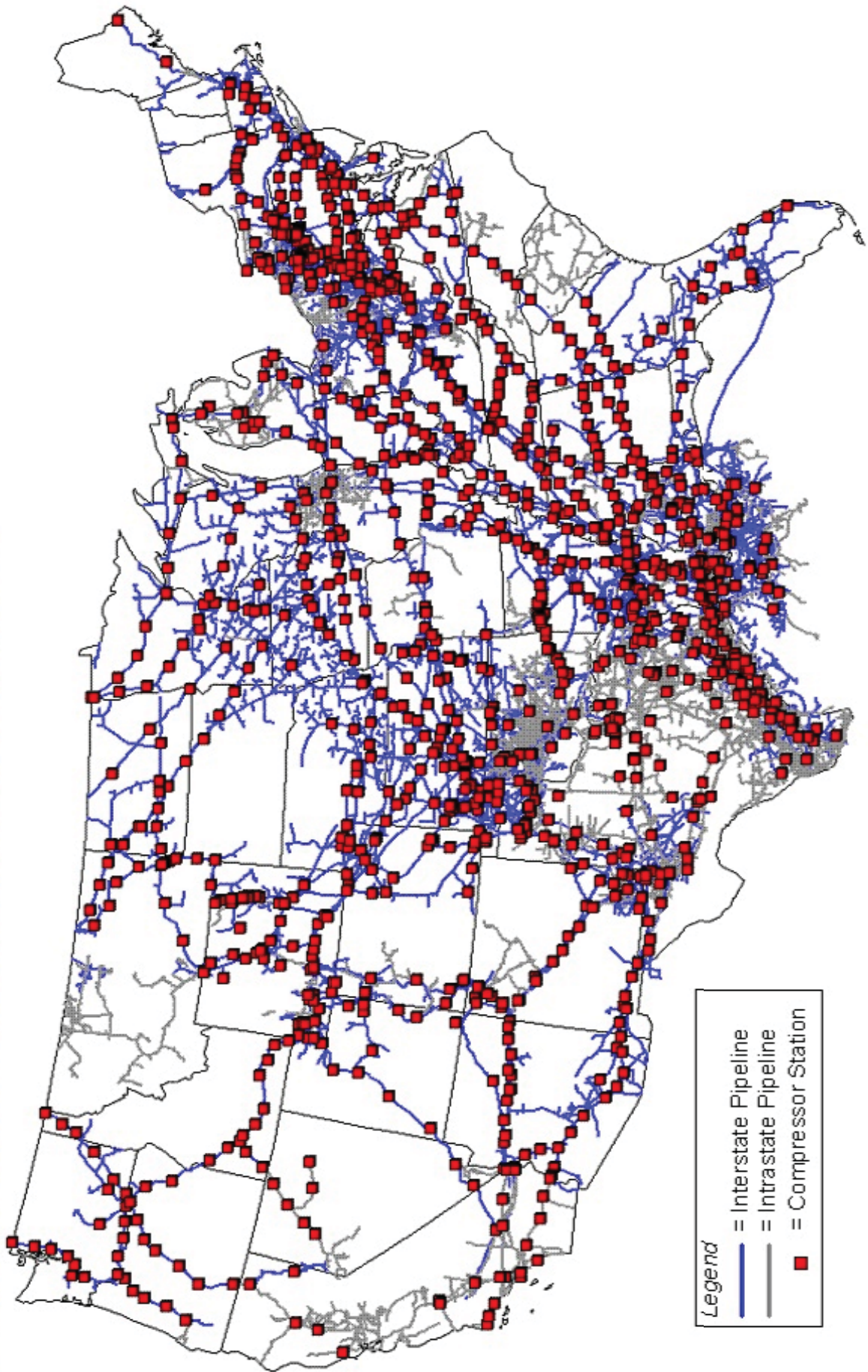
U.S. Natural Gas Pipeline Compressor Stations Illustration, 2008
