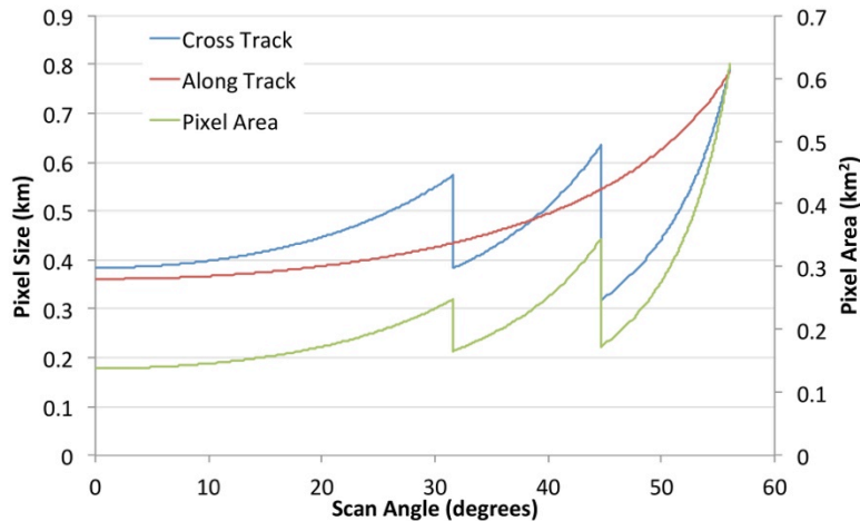
Figure 1: Spatial resolution of VIIRS imager data as a function of scan angle. The three distinct regions represent unique data aggregation zones extending from nadir to the edge of the swath.
