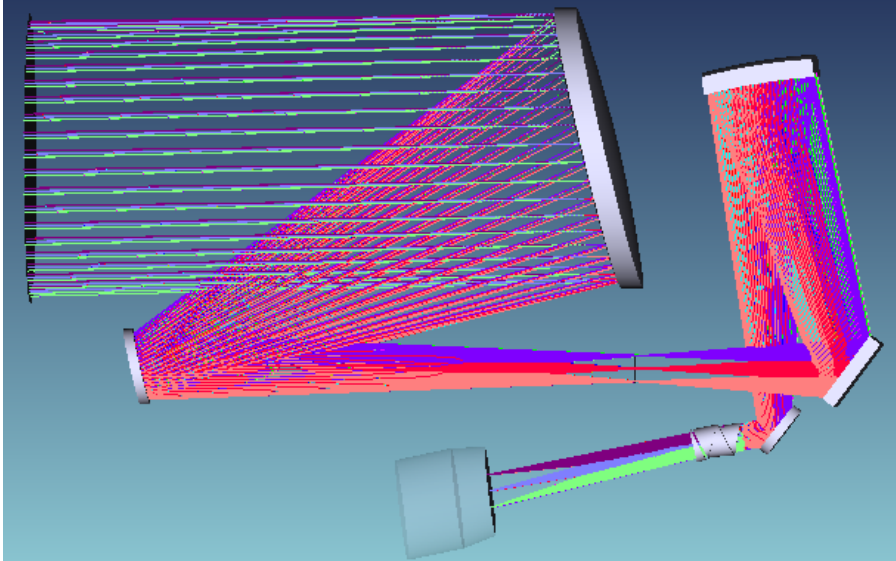
Optical ray trace layout for H2E1
