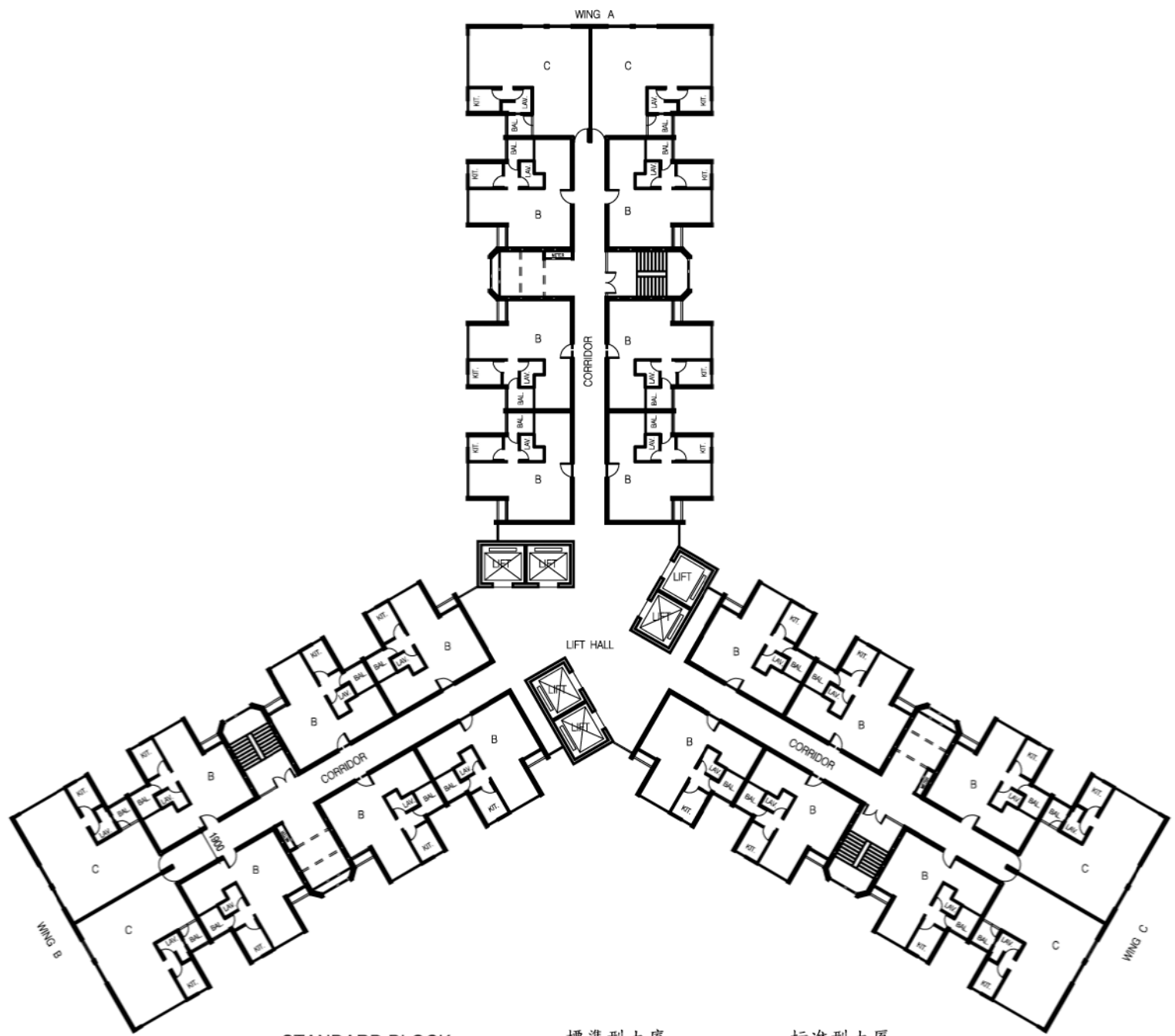
STANDARD BLOCK TRIDENT 2 (35-STOREY) TYPICAL FLOOR PLAN
