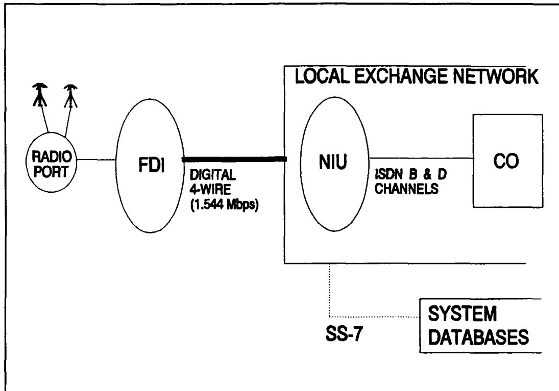
Figure 16. Bellcore PCS Standard Interfaces
