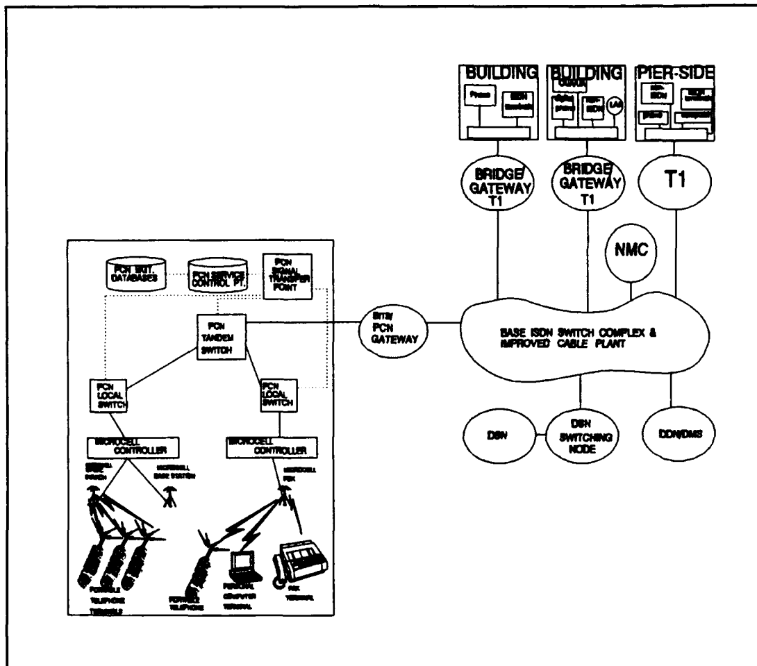
Figure 20. Target BITS Architecture/Wireless
