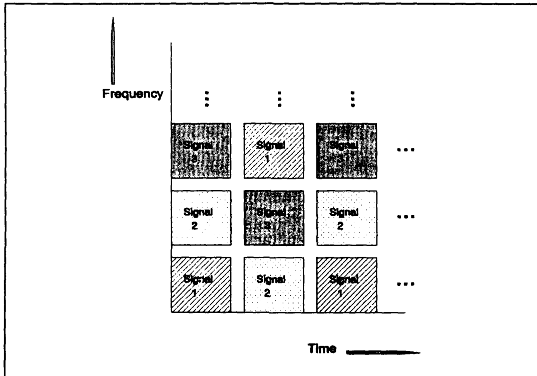
Figure 13. FH-CDMA [Ref. 33: p. 491]
