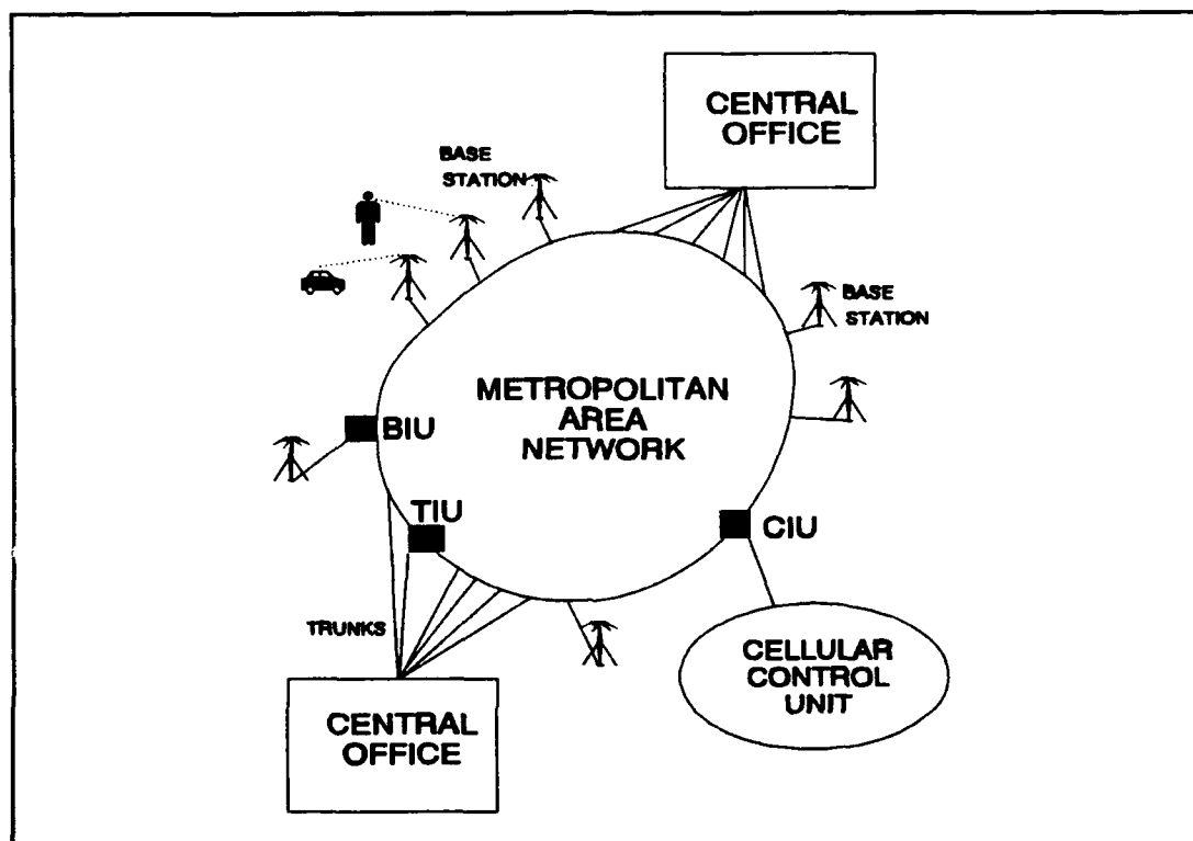
Figure 18. Cellular Packet Switch [Ref. 22:p. 1274]
