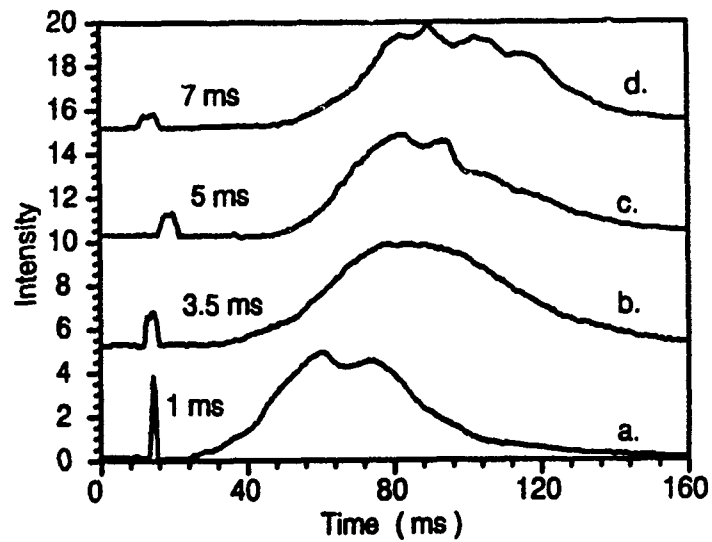
Figure 9. Effect of Laser Pulse Duration on Blackpowder Ignition Delay at Constant Laser Energy (2 J).
