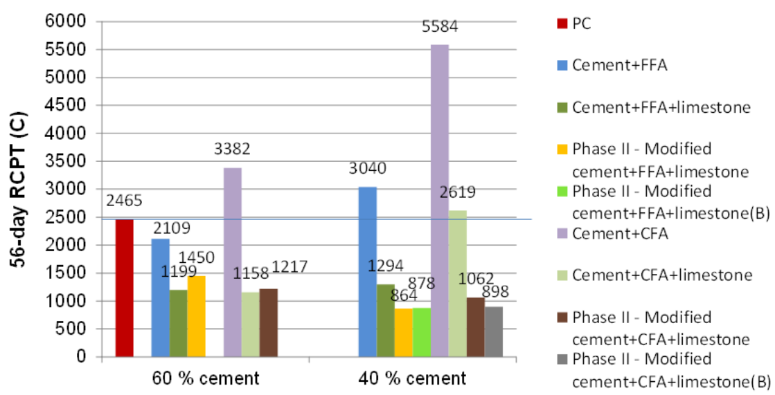
Figure 14. Measured cumulative charge passed (RCPT) at 56 d for the 15 concrete mixtures (taken from [65]). Coefficients of variation for three replicate specimens varied from 2.1 % to 19.1 % for the various mixtures.
