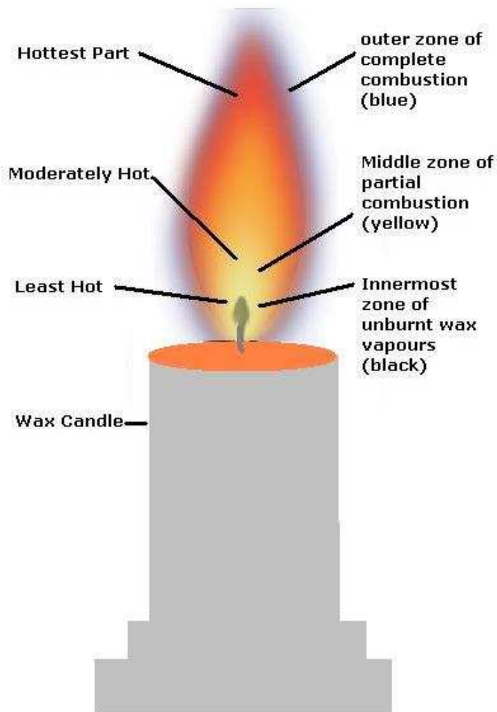
Labelled diagram of Different Zones of Candle flame
