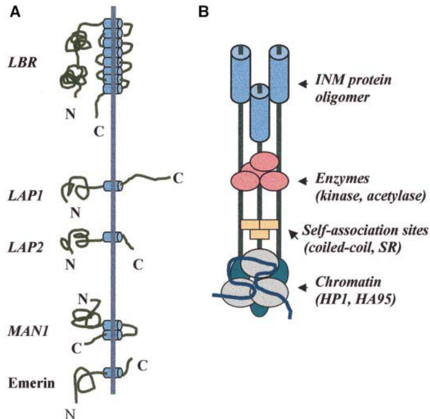
Fig. 1. Topology and organization of inner nuclear membrane proteins. (A) Schematic diagram depicting the structural and topological features of the currently known integral proteins of the inner nuclear membrane. The hydrophilic end-domains (irregular lines) project to the nucleoplasm (left) and the perinuclear space (right), while the membrane-spanning regions (barrels) cross the inner nuclear membrane (straight line). (B) A highly hypothetical model of inner nuclear membrane complexes. The aggregate is postulated to contain oligomers of membrane proteins (held in place via coiled-coiled or SR-SR interactions), modulating enzymes and chromatin-associated elements.
