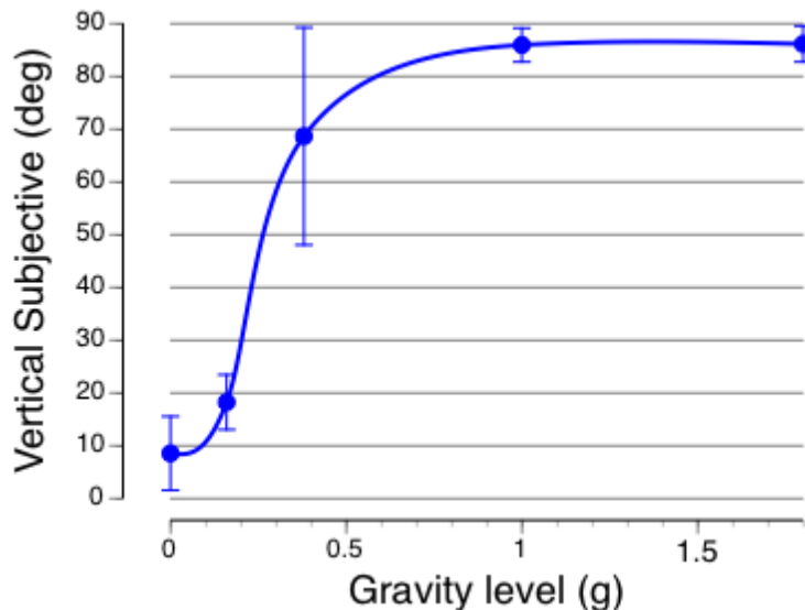
Figure 4. Dose-response curve of perception of verticality versus gravity level in parabolic flight. Mean of 6 subjects, 15-60 trials per subjects. Subjects lying on their side were able to accurately align their subjective vertical with the gravitational vertical for gravity levels ranging from 0.3 g to 1.8 g. Below 0.3 g they aligned their subjective vertical with their long body axis. Adapted from Winkel et al. (2012).
