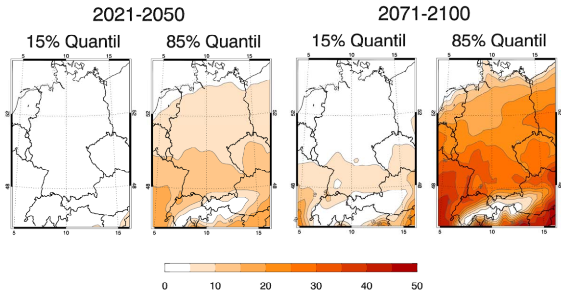
Fig. 6: Projected change in the number of hot days ( T_{\max} \geq 30^\circ\text{C} ), means for the projection periods 2021-2050 (left) and 2071-2100 (right). For details of the climate projections used, see Figure 4.
