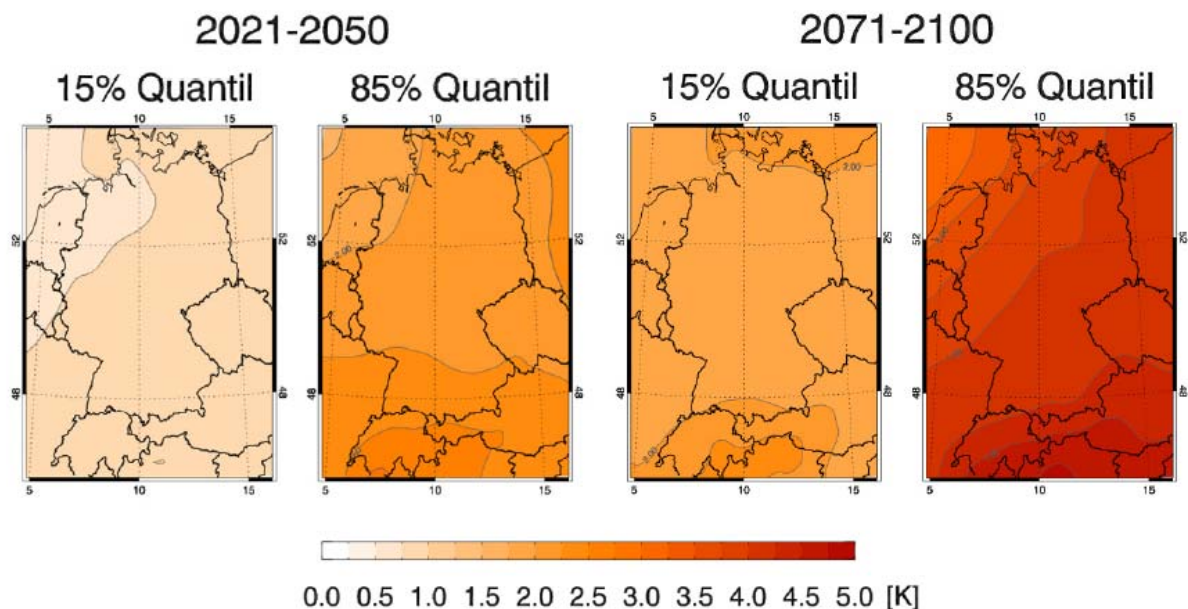
Fig. 5: Projected change in annual mean air temperature, means for the projection periods 2021-2050 (left) and 2071-2100 (right). For details of the climate projections used, see Fig. 4.
