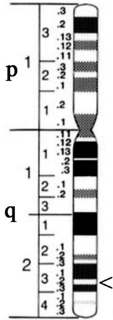
Figure 1. Human Chromosome #16
