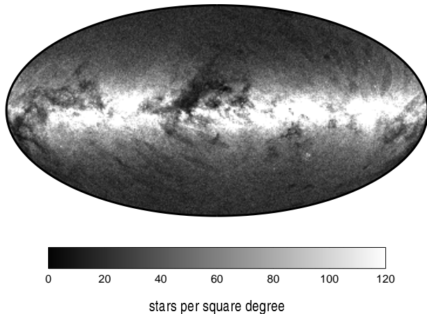
Fig. 1. The Tycho-2 Catalogue: number of observed stars per square degree, in galactic coordinates centred at l = 0 . In some areas the density is above 400 \text{ stars deg}^{-2} , with a maximum of 450. The average density is 150 \text{ stars deg}^{-2} at b = 0 and decreases to 25 \text{ stars deg}^{-2} at |b| = 90^\circ . Traces of the Hipparcos scanning pattern appear as stripes with lower star density.
