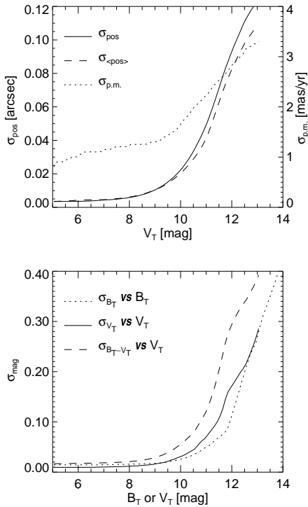
Fig. 2. The Tycho-2 Catalogue accuracy. (a): Standard errors of the observed position components, of the mean position at mean epoch, and of proper motion components; (b): standard errors of magnitudes and colour indices versus B_T or V_T (see also Table 2).
