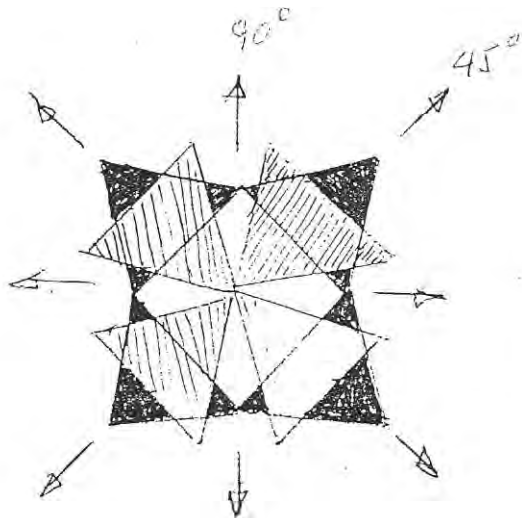
GRAVITATIONAL AND MAGNETIC FIELDS
