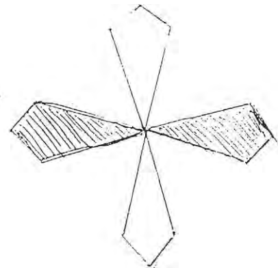
MAGNETIC FIELD
