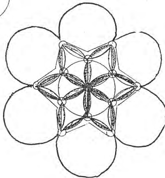
ELECTRONS OR- BITAL PATH WHEN IN LOCKSTEP AND PAIRED IN SACRED GEOMETRY, IN SUCH A SYSTEM, ALL PHOTONS WITHIN THE ELEC- TRON (ELECTRONS MADE OF PHOTOS) ALSO PRESENT IN ORDERED FORM.
