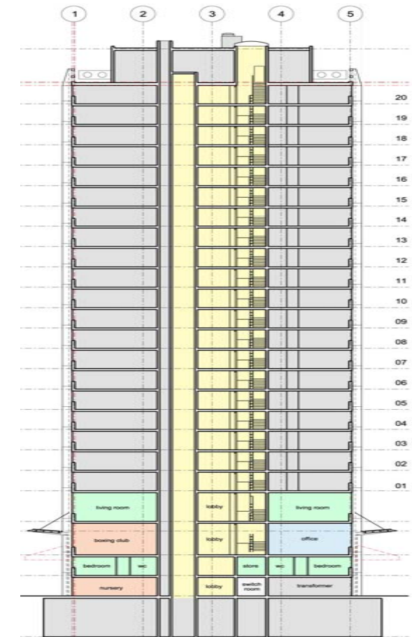
15 Cross section showing reconfigured areas at podium level coloured
