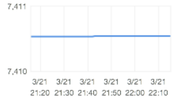
CPUCreditBalance (Count)
