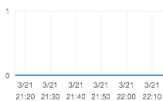
AutomatedSnapshotFailure
