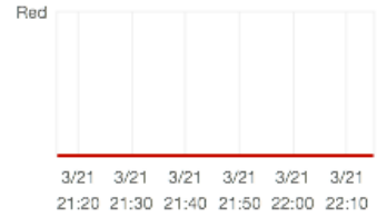
ClusterStatus.red
