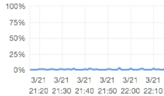
JVMMemoryPressure (Percent)
