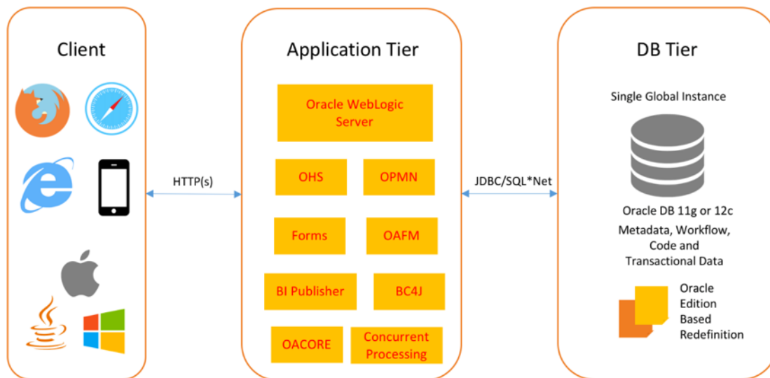
Figure 3: Oracle E-Business Suite three-tier architecture
