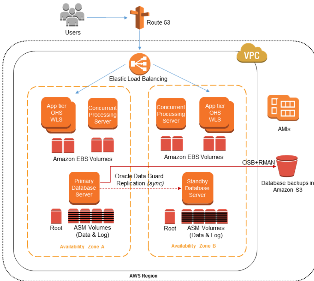
Figure 4: Sample Oracle E-Business Suite deployment on AWS
