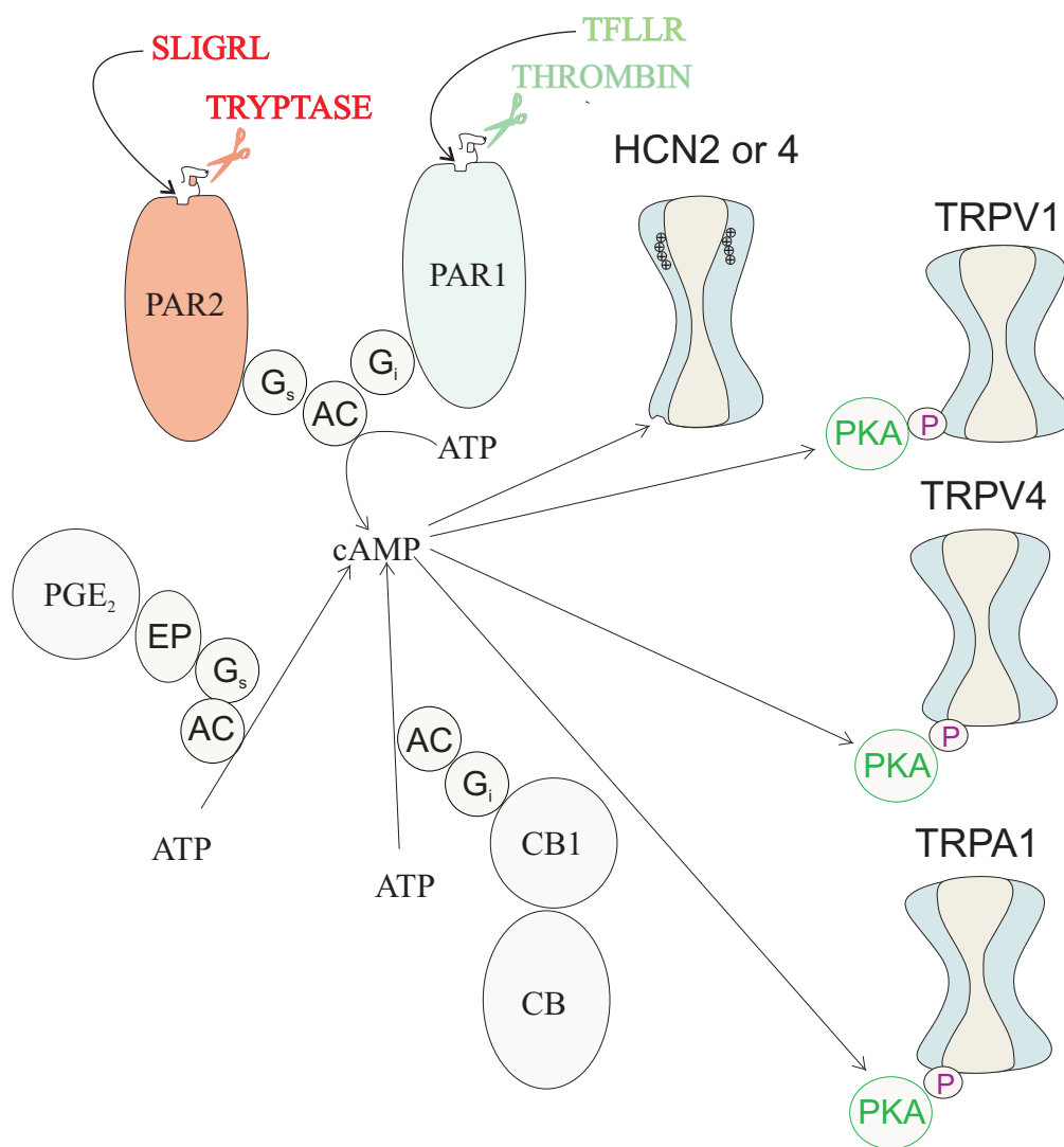
Figure 6-3. Regulation of nociceptor function by cAMP and PKA. PAR2 and PGE 2 activate AC via G s thereby leading to an increase in cAMP concentration and thereby to activation of PKA. In contrast PAR1 and CB1 inhibit AC via G i thereby leading to a decrease in cAMP concentration and a decrease in the activity of PKA.
