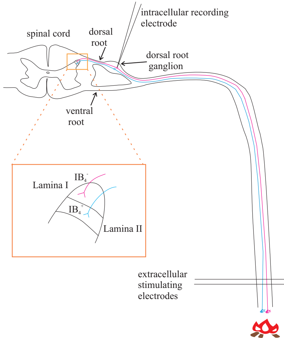
Figure 1-1. Intense heat from a fire activates the terminals of two nociceptors. Action potentials are propagated along the axons of the nociceptors into the spinal cord and the activity of one of the nociceptors is monitored by an intracellular electrode which impales its cell body which is located in the dorsal root ganglion (DRG). The central terminal of a fiber staining positive for the plant lectin isolectin B4 ( IB_4^+ ) is shown terminating in lamina II and that of an IB_4^- fiber is shown terminating in lamina I. The extracellular stimulating electrodes are connected to a pulse stimulator (not shown) and are used to initiate action potentials in the nerve fibers.
