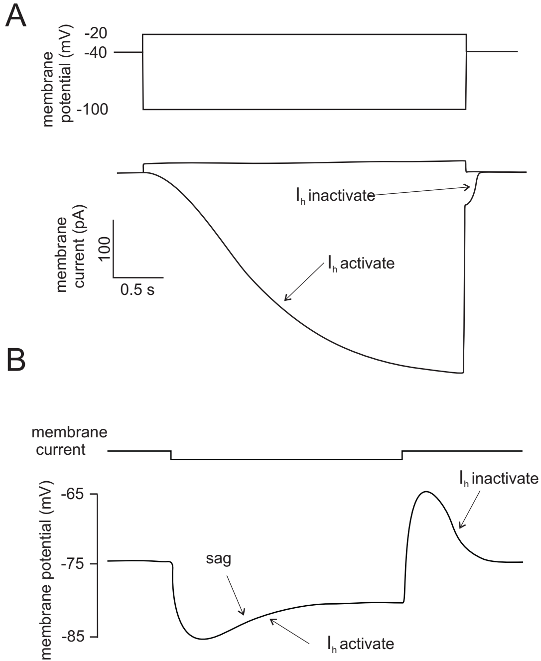
Figure 5.2. I_h activation and inactivation under voltage clamp (A) and current clamp (B) conditions. In (A) I_h is activated by a voltage step from -40 to -100 mV and inactivates when the voltage returns to -40mV. In (B) a hyperpolarizing current pulse activates I_h causing a depolarizing sag during the membrane hyperpolarization.
