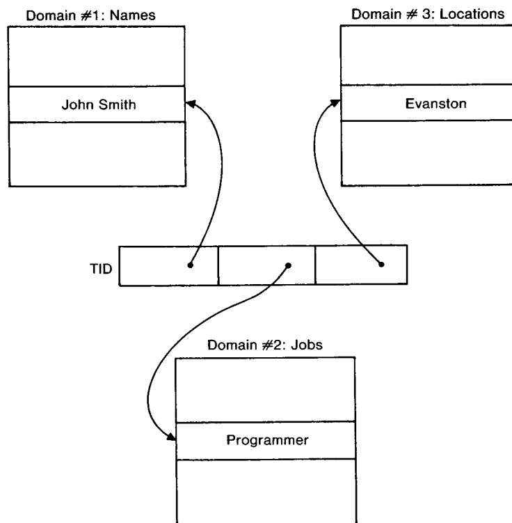
Fig. 2. XRM Storage Structure.
