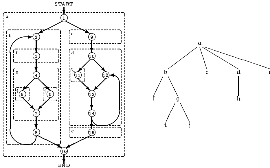
Figure 5.7: SESE regions and PST for the CFG of Figure 5.5 (from [19]).
