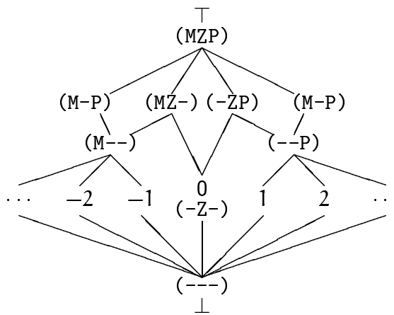
Figure 6.11: An integer lattice for signed integers. A classification into negative (M), positive (P), or zero (Z) is grafted onto the standard flat integer constant domain. The (M-P) entry is duplicated to aid clarity.
