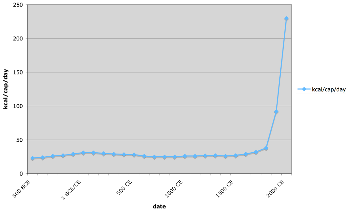
Graph 10. Western energy capture, 500 BCE-2000 CE
