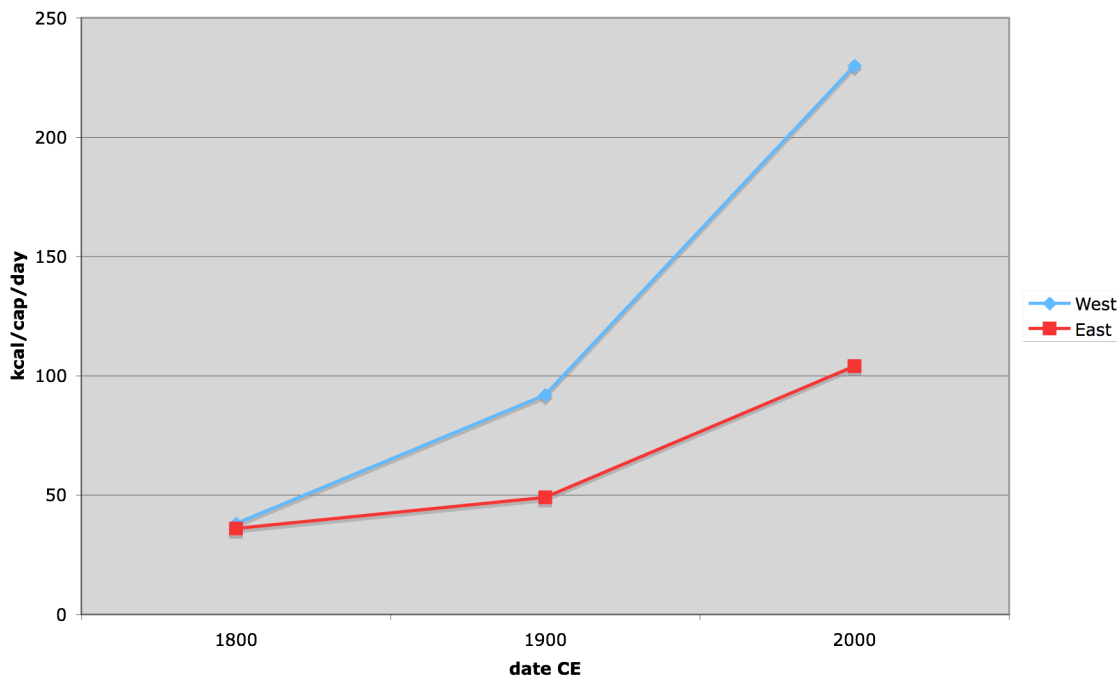
Graph 21. Eastern and Western energy capture, 1800-2100 CE
