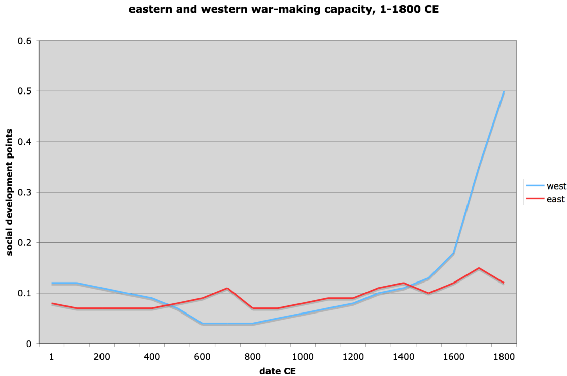
Graph 50. Eastern and Western war-making capacity, 1-1900 CE
