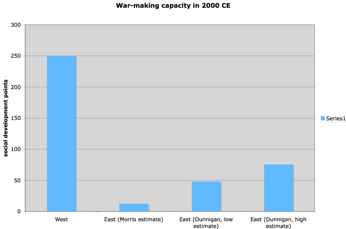
Graph 53. Alternative quantitative estimates of the East: West military balance, 2000 CE
