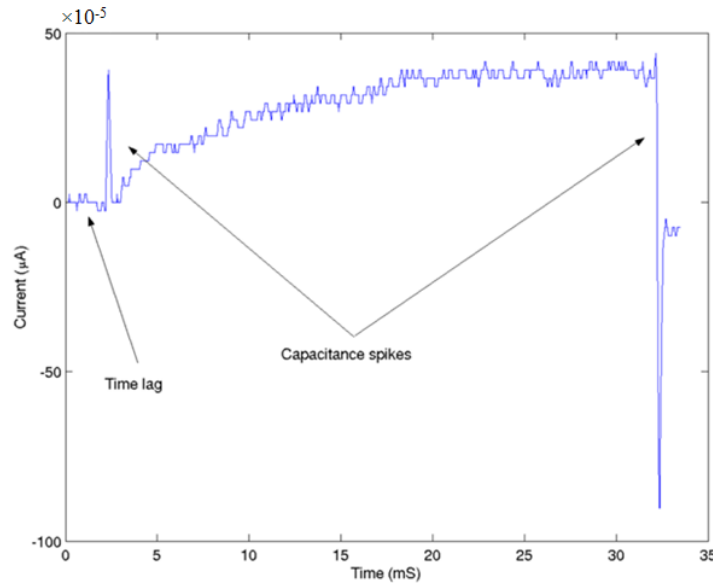
Figure 1. K^+ current in a gonadotroph cell, when the holding voltage is stepped from -10 mV to +116 mV using a voltage clamp. We modified this data before we used it ourselves, removing the labelled capacitance spikes and time lag. We repeated this action for all other current data used. The x -axis presents time (mS); the y -axis presents K^+ current.
