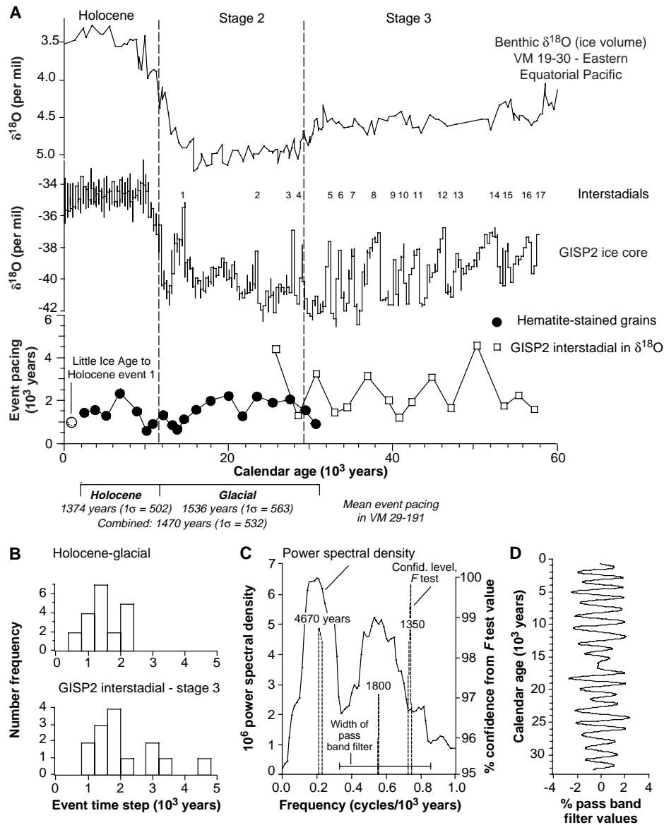
Fig. 7. (A) Time series of pacings of Holocene-glacial events from VM 29-191 and VM 23-81 (●), compared with pacings of numbered interstadials in GISP2 \delta^{18}\text{O} (□) and benthic \delta^{18}\text{O} in VM 19-30 (66). Pacings were calculated as in (27). The pacings of the Dansgaard/Oeschger cycles were obtained by measuring the time steps between numbered interstadials and placing the value at the midpoints between them. The time step to the Little Ice Age (○) is also shown for comparison with older event pacings. Mean values of event pacings are from the composite record of hematite-stained grains in Fig. 6. The calibrated time scale for VM 19-30 is from (25). On the basis of radiocarbon ages and their calibrations, the stage 2–stage 3 boundary is almost 6000 years older than given by SPECMAP tuning (67). (B) Histogram of Holocene-glacial IRD events and GISP2 interstadial events. (C) Multitaper spectral analysis (7 tapers) of time series of hematite-stained grains. (D) Filtered record of time series of hematite-stained grains.
