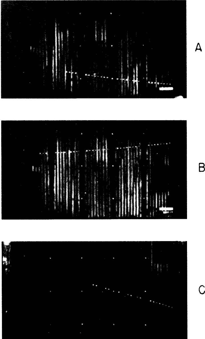
Figure 5. Some typical single muon events.
