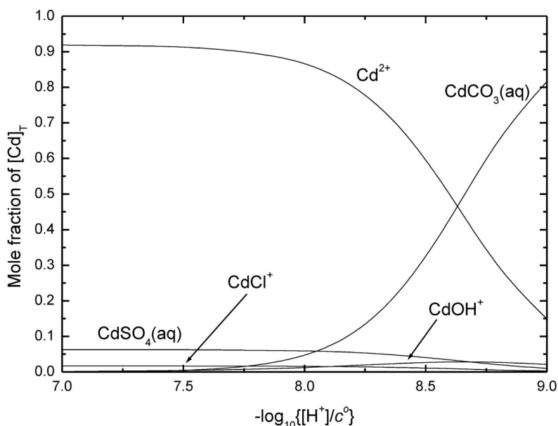
Fig. 5 Speciation diagram for the \text{Cd}^{2+} + \text{H}^+ + \text{Cl}^- + \text{CO}_2 + \text{HPO}_4^{2-} + \text{SO}_4^{2-} system with total concentrations [\text{Cl}^-]_T = 0.23 \text{ mmol dm}^{-3} , [\text{SO}_4^{2-}]_T = 0.42 \text{ mmol dm}^{-3} , [\text{HPO}_4^{2-}]_T = 0.7 \text{ } \mu\text{mol dm}^{-3} (fresh water medium) and [\text{Cd}^{\text{II}}]_T = 1 \text{ nmol dm}^{-3} . It was assumed that the system is in equilibrium with air having a \text{CO}_2 fugacity of 370 \mu\text{bar} . \text{Log } K_{10}(\text{CO}_2(\text{g}) = \text{CO}_2(\text{aq})) = -1.5 [93MOR]. All other formation constants are according to Table 6 ( I_c = 0.0015 \text{ mol dm}^{-3} ).
