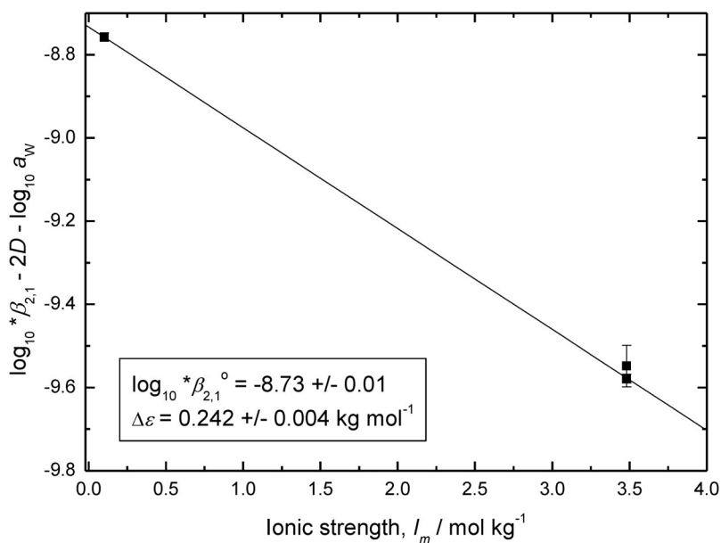
Fig. A3-4 Extrapolation to I_m = 0 \text{ mol kg}^{-1} of \log_{10} \beta_{2,1}^* - \Delta(z^2)D - \log_{10} a(\text{H}_2\text{O}) for reaction 9 ( \Delta z^2 = 2 ) using selected data for perchlorate media, 25 °C (Table A2-4).
