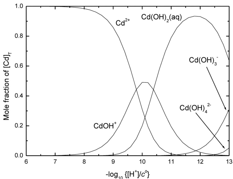
Fig. 1 Speciation diagram for the binary \text{Cd}^{2+} + \text{OH}^- system as obtained from the Recommended stability constants at 25^\circ\text{C} and I_m = 0 \text{ mol kg}^{-1} (Table 1) and calculated for [\text{Cd}^{\text{II}}]_{\text{T}} = 1 \times 10^{-6} \text{ mol dm}^{-3} . Results with -\log_{10}\{[\text{H}^+]/c^\circ\} greater than 12 should be viewed with caution as activity coefficients deviate from 1.0. No corrections were made for ionic strength-dependent changes in formation constants at high pH.
