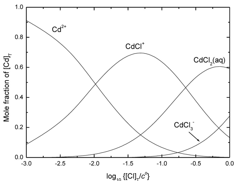
Fig. 2 Speciation diagram for the binary \text{Cd}^{2+} + \text{Cl}^- system as obtained from the Recommended stability constants at 25^\circ\text{C} and I_m = 0 \text{ mol kg}^{-1} (Table 2) and calculated for [\text{Cd}]_{\text{T}} = 10^{-6} \text{ mol dm}^{-3} , assuming -\log_{10} \{[\text{H}^+]/c^\circ\} < 7.5 , and with no corrections made for ionic strength-dependent changes in formation constants.
