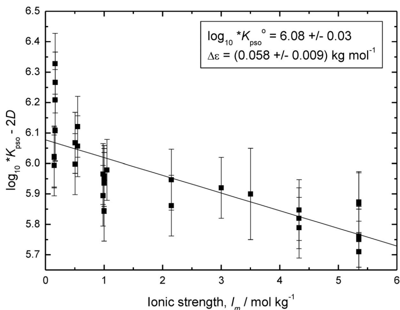
Fig. A3-11 Extrapolation to I_m = 0 \text{ mol kg}^{-1} of \log_{10} *K_{\text{ps0}}^0 - \Delta(z^2)D for reaction 29 ( \Delta z^2 = 2 ) using selected data for perchlorate media, 25 °C (Table A2-12).
