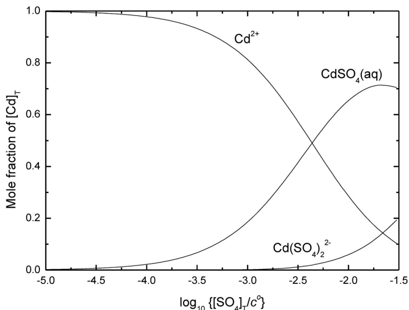
Fig. 4 Speciation diagram for the ternary \text{Cd}^{2+} + \text{SO}_4^{2-} system as obtained from the Recommended and Provisional stability constants at 25^\circ \text{C} and I_m = 0 \text{ mol kg}^{-1} (Table 4), calculated for [\text{Cd}]_T = 10^{-6} \text{ mol dm}^{-3} . No corrections were made for ionic strength-dependent changes in formation constants.
