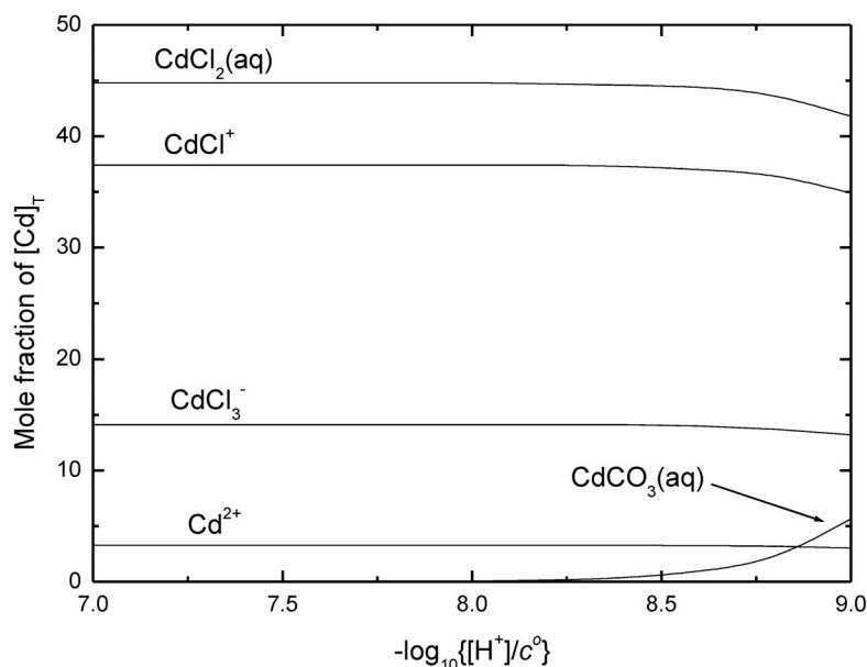
Fig. 6 Speciation diagram for the \text{Cd}^{2+} + \text{H}^+ + \text{Cl}^- + \text{CO}_2 + \text{HPO}_4^{2-} + \text{SO}_4^{2-} system in a simulated seawater medium, I_c = 0.67 \text{ mol dm}^{-3} including carbonato- and sulfato- complexes of \text{Mg}^{2+} and \text{Ca}^{2+} . It was assumed that [\text{Cd}^{\text{II}}]_{\text{T}} = 1 \text{ nmol dm}^{-3} and that the system is in equilibrium with air having a \text{CO}_2 fugacity of 10^{-3.5} bar. \text{Log } K_{10}(\text{CO}_2(\text{g}) = \text{CO}_2(\text{aq})) = -1.5 [93MOR]. All other formation constants are according to Table 6 ( I_c = 0.67 \text{ mol dm}^{-3} ).
