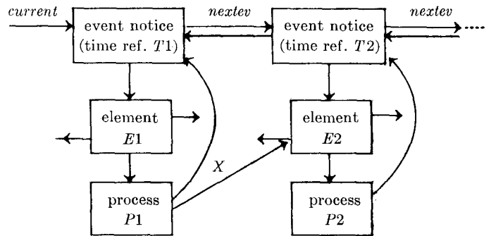
Fig. 3. The sequencing set. P1 is the currently active process, P2 is suspended, "current" is equal to E1 and "time" is equal to T1 . P1 has a local element variable X , to which has been assigned the value "nextev(current)". "evtime( X )" is equal to T2 , which is greater than or equal to T1 .
