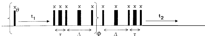
Figure 19. Pulse sequence for C, spin topology filtration consisting of \pi/2 and \pi pulses. The delays are adjusted to \tau = 1/(8J) and \Delta = 1/(2J) where J is the uniform J-coupling constant. \Phi is phase-cycled for four-quantum selection and \Theta for the suppression of axial peaks (94).
