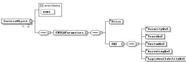
Figure 9. The details of ServiceObject
