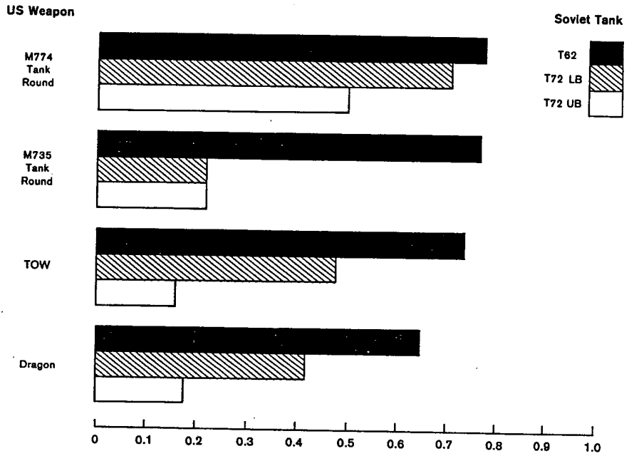
Probability of Kill Given Hit, Firer and Target Stationary, Target Fully Exposed, 0° Azimuth (Front)
