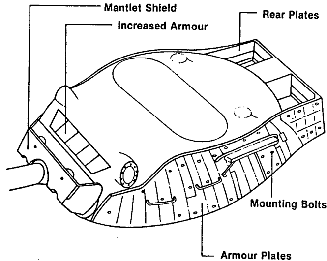
Figure 26. FRG Leopard Tank with Zuzatzpanzerung
