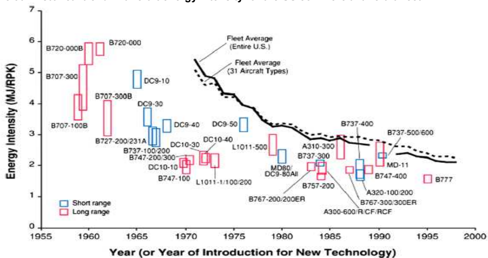
Figure 30: Historical trend in aircraft energy intensity for the US commercial aircraft fleet 73
