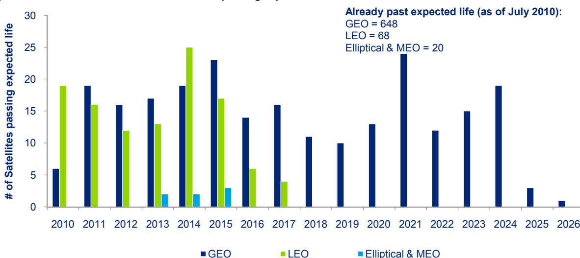
Figure 37: Number of listed launched satellites passing expected useful life 118
