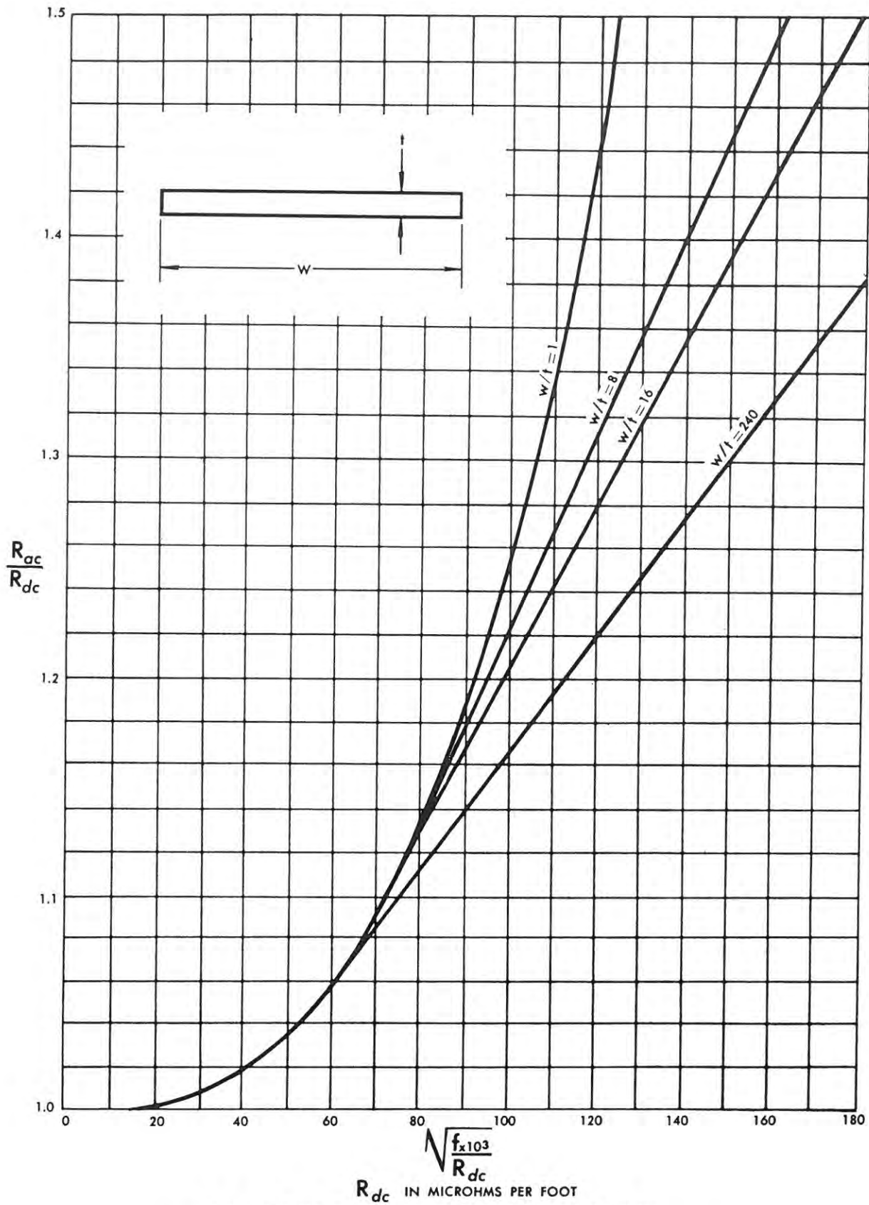
Fig. 13-6. Curves for skin effect of isolated flat rectangular conductors.
