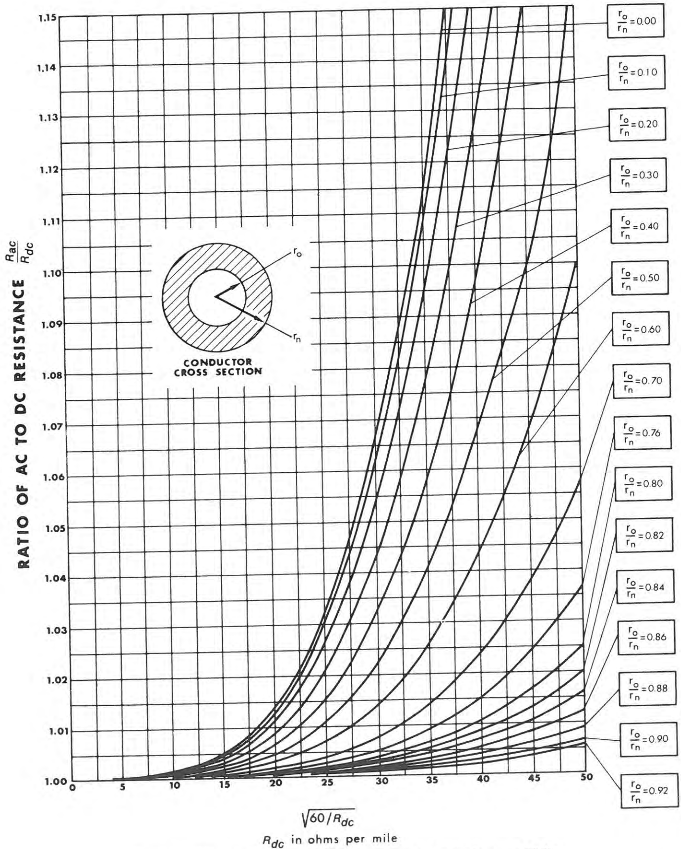
Fig. 3-8. Skin-effect factor for solid-round or tubular conductor at 60 Hz.
