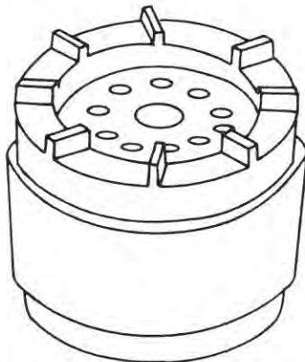
Fig. 16-2. A typical die-cast rotor of the open-slot type.
