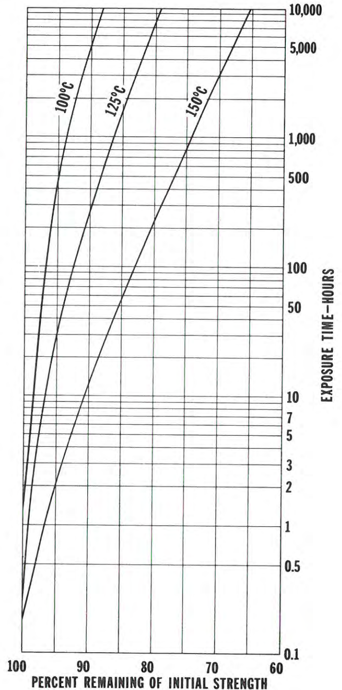
Fig. 6-3. Time-temperature percent strength remaining in 1350-H19 wire. Tensile tests made at room temperature after wire exposure to the indicated temperatures.
