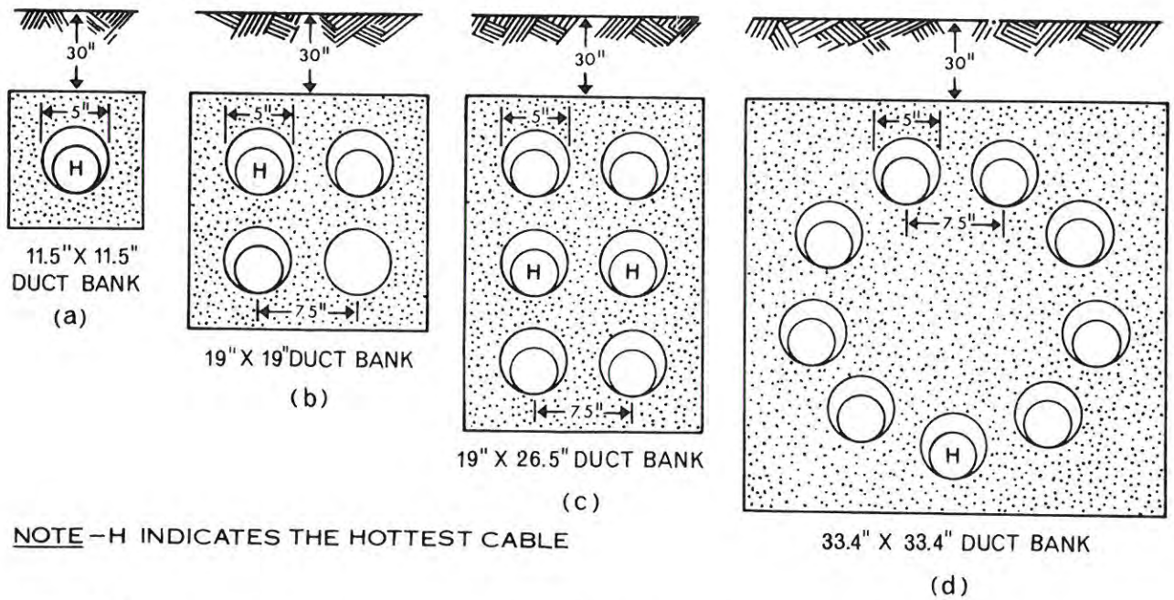
Fig. 9A-1. Arrangements of 1, 3, 6, and 9 cables in underground duct, as basis for ampacity calculations.
