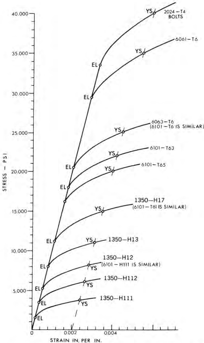
Fig. 13-3. Approximate tension stress-strain curves at 70°C on guaranteed minimum basis for aluminum bus conductor alloys—½ in. thickness bus bars and ½ in. diam. 2024-T4 bolts. Yield strength (YS) is arbitrary at 0.2% offset per ASTM Standard. Elastic limit is estimated as point of tangency (EL).
