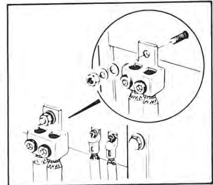
Fig. 11-12. Copper lug connections on switchgear are replaced with equivalent aluminum connectors. Belleville washer is used with copper or steel studs.
