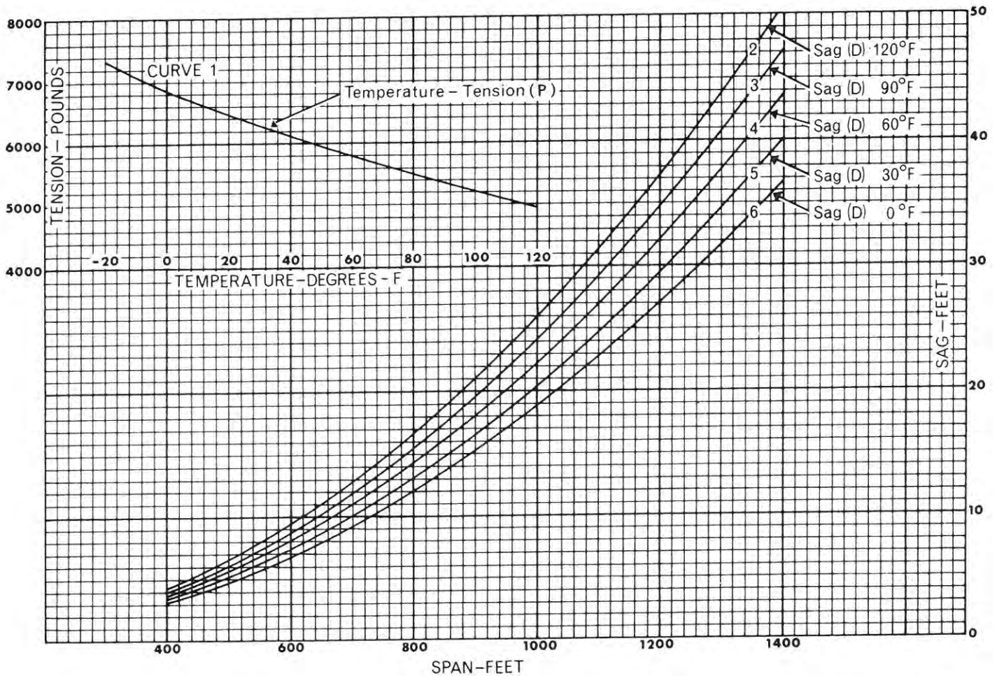
Fig. 5-4. Initial Stringing Chart. Stringing sags and tensions for constant tension at a given temperature for a 795 kcmil 54/7 Condor ACSR. For Ruling Span of 1,000 ft and 11,280 lb maximum initial tension with heavy loading. There is no loading during initial stringing, hence tension is per curve 1.
