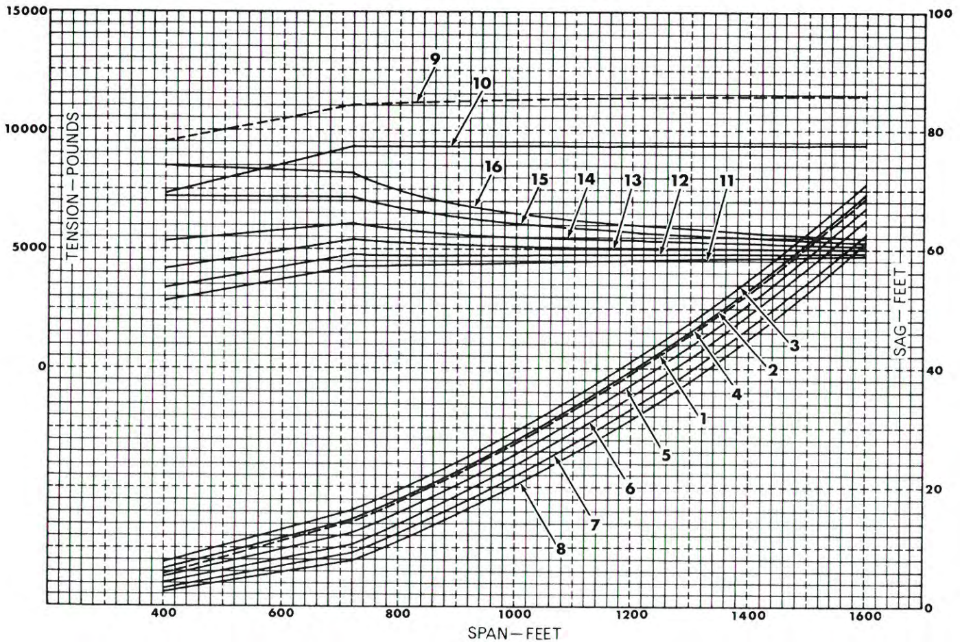
Fig. 5-3. Sags and tensions, final. 795 kcmil, 54/7 Condor ACSR.
