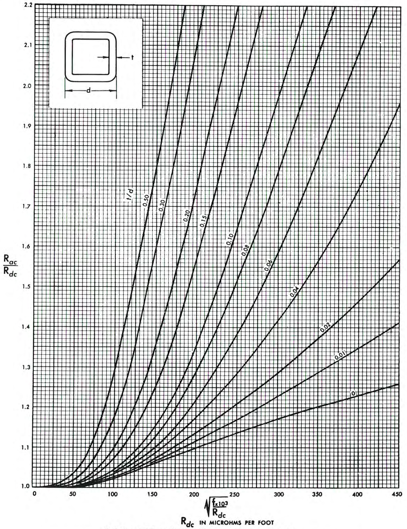
H. B. Dwight, "Electrical Coils and Conductors," McGraw-Hill Book Co. Fig. 13-7. Curves for skin effect of isolated square rod and square tubular conductors.
