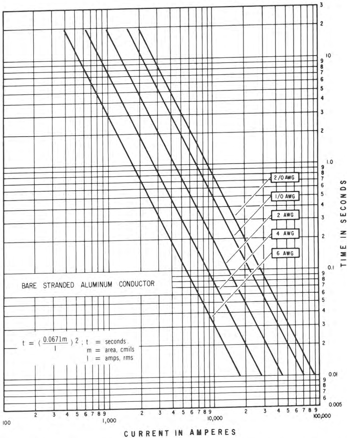
Fig. 6-1A. Maximum fault-current operating limit for stranded aluminum conductor. Upper temperature limit 340°C, ambient temperature 40°C.
