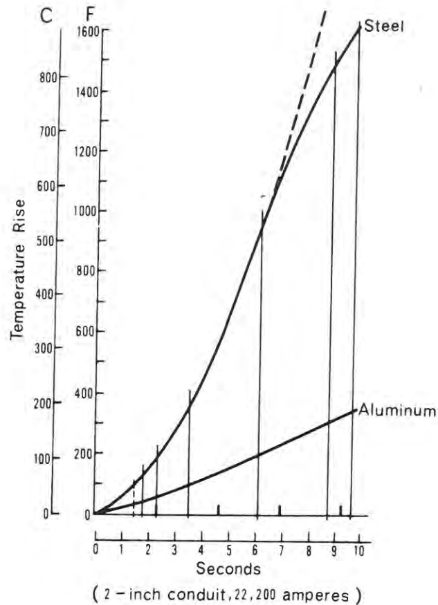
Fig. 17-1. Measured temperature rise vs time for aluminum and steel conduit under short circuit conditions.
