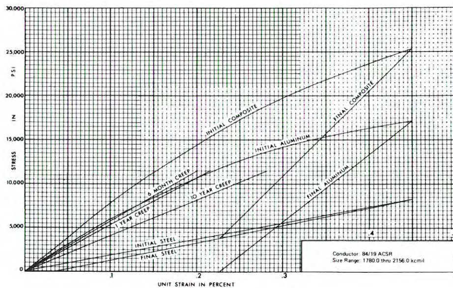
Fig. 5-17. Stress-Strain Curves.
