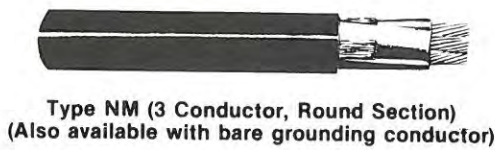
Fig. 10-8. Type NM branch-wiring cables.
