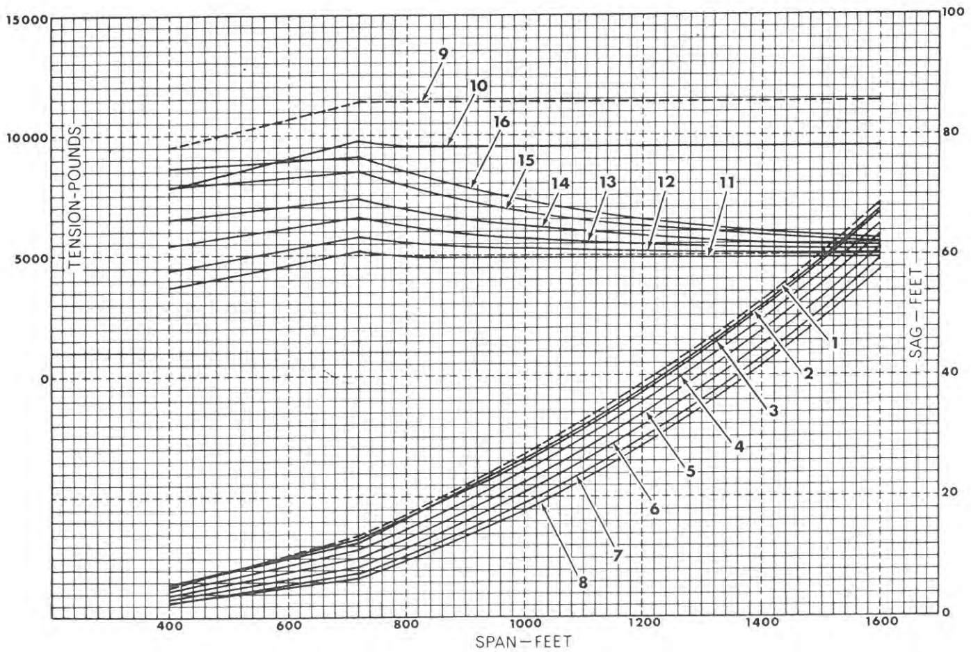
Fig. 5-2. Sags and Tensions, Initial. 795 kcmil, 54/7 Condor ACSR.
