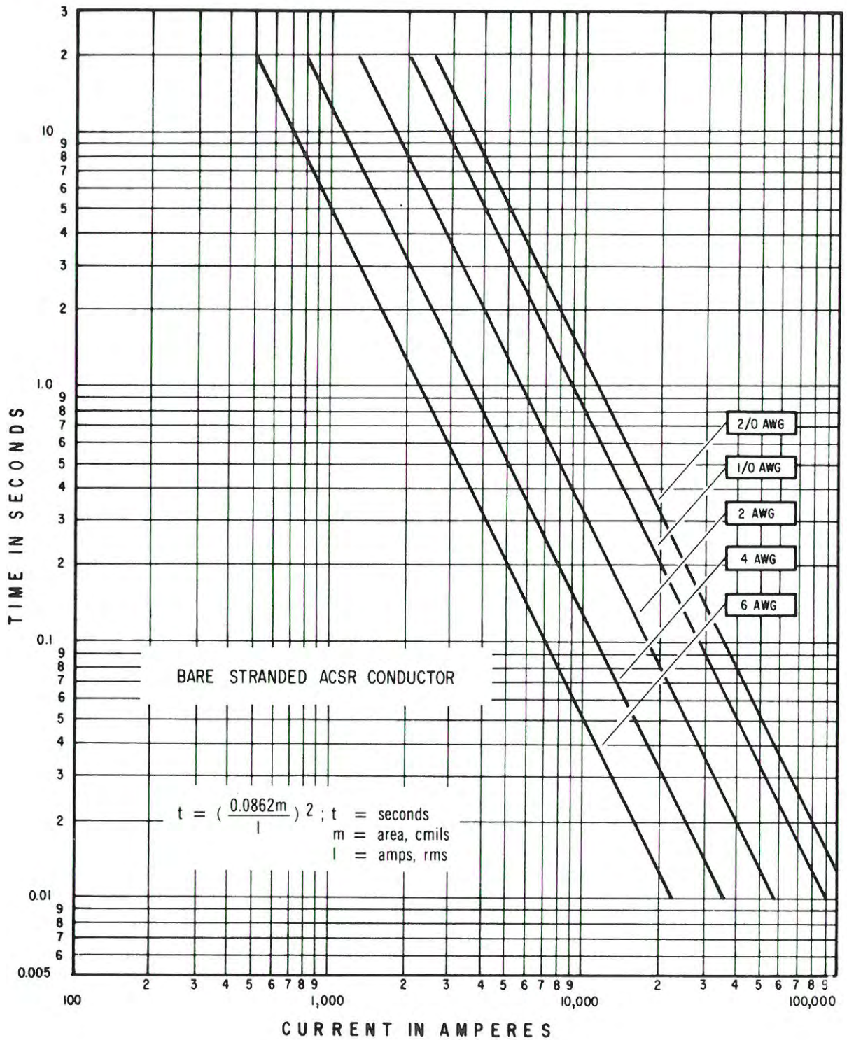
Fig. 6-2A. Maximum Fault-Current Operating Limit for Bare Stranded ACSR conductor. Upper temperature limit 645°C, ambient temperature 40°C.
