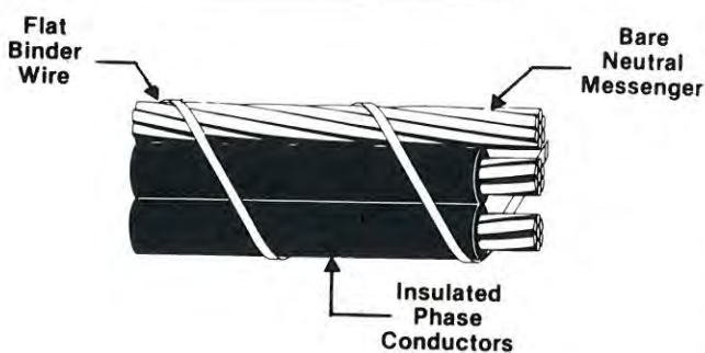
Fig. 10-2. Preassembled parallel secondary cable.
