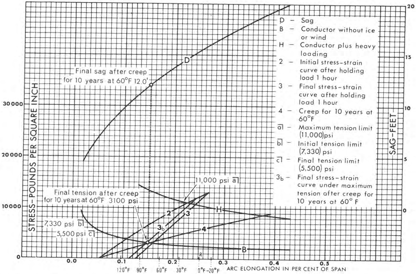
Fig. 5-14. Final trial for 0°F after adjustment for 10-year creep correction. Values for 0°F unloaded, and 0°F with heavy load are entered from this graph on Table 5-5.
