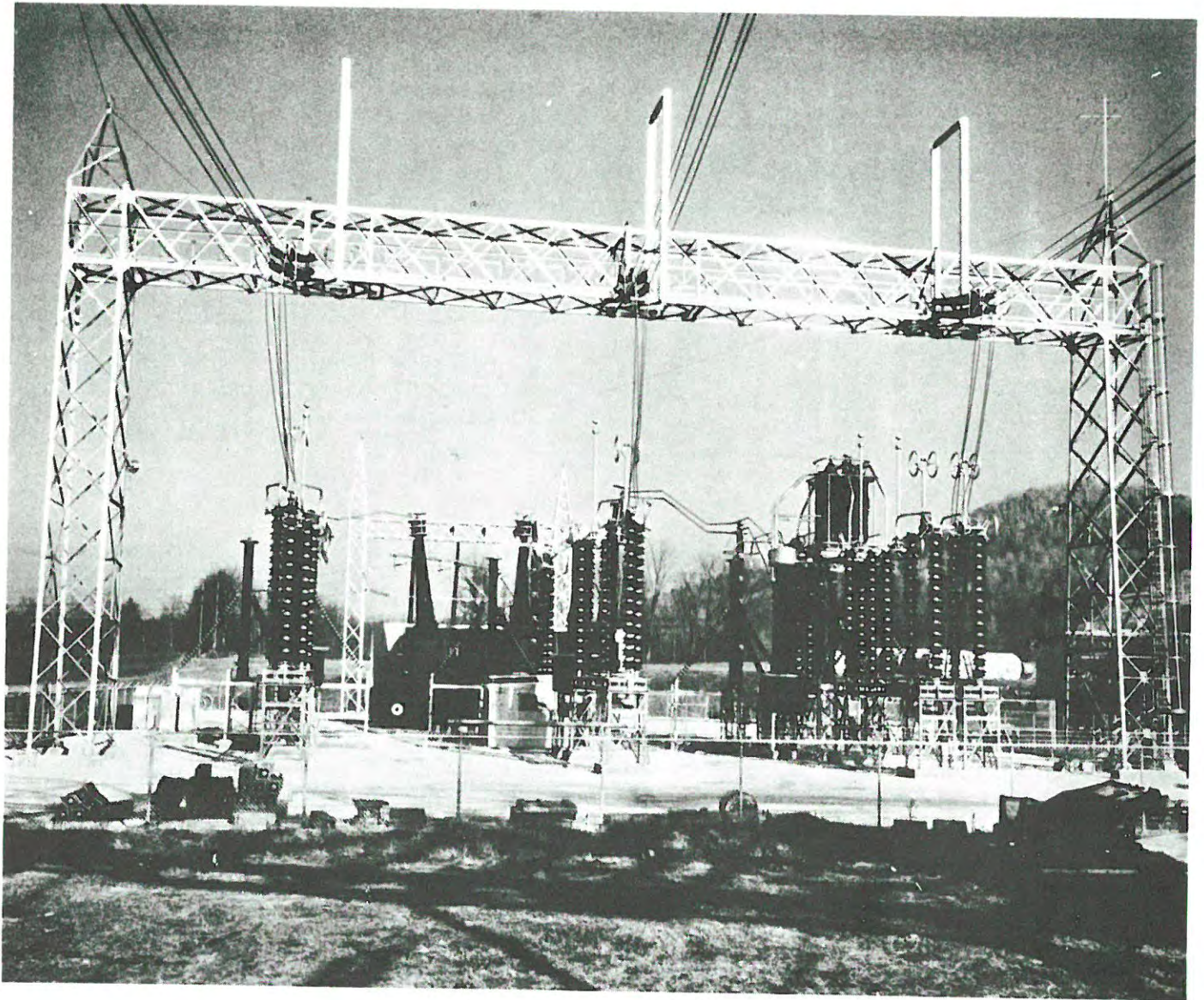
Fig. 18-13. All-aluminum substation designed to operate at 750 kV.
