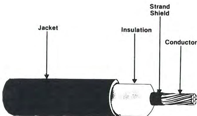
Fig. 10-12. Typical unshielded aluminum insulated primary cable 5 kV with jacket.
