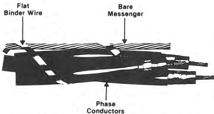
Fig. 10-14. Typical pre-assembled triplexed 5-kV to 25-kV shielded primary cable bound to composite aluminum-steel (ACSR or ACSR/AW) or aluminum-alloy messenger with aluminum tape. A fourth insulated neutral may be included if required.
