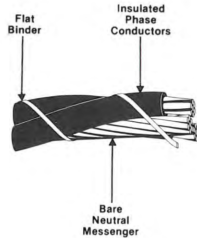
Fig. 10-3. Preassembled reverse lay twist cable.
