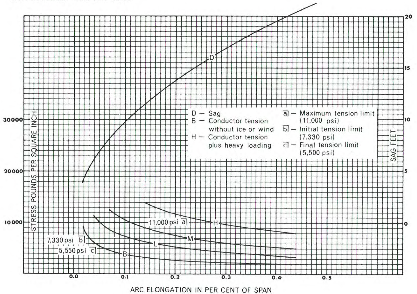
Fig. 5-11. Preliminary Sag-Tension Graph.
