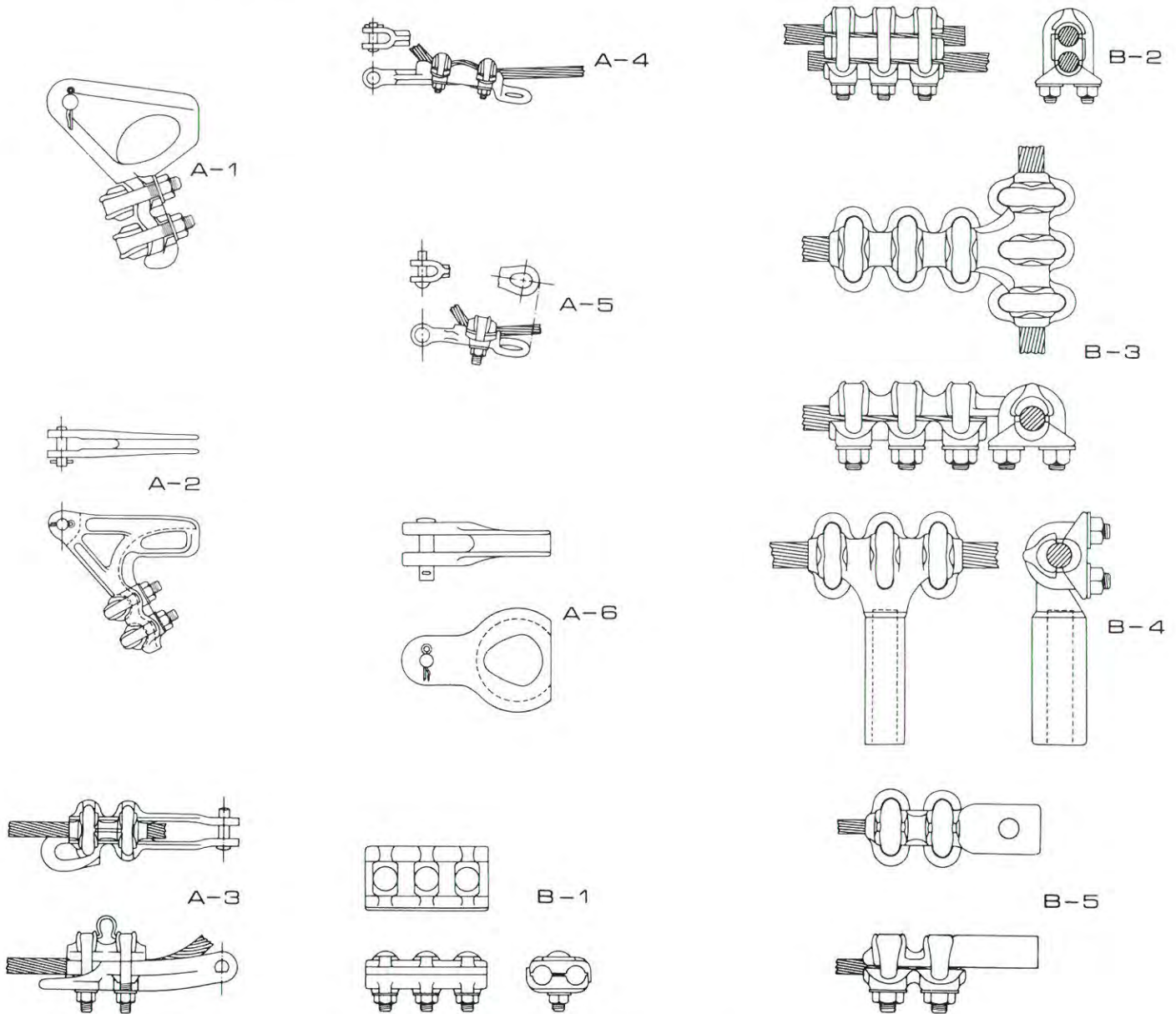
Fig. 5-21. Clamp-bolt connections.
