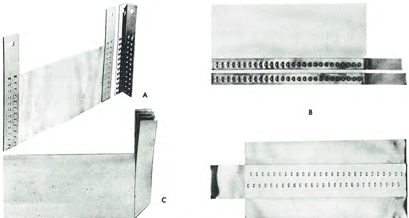
Fig. 14-7. Various methods of applying terminals to aluminum strip conductor.
