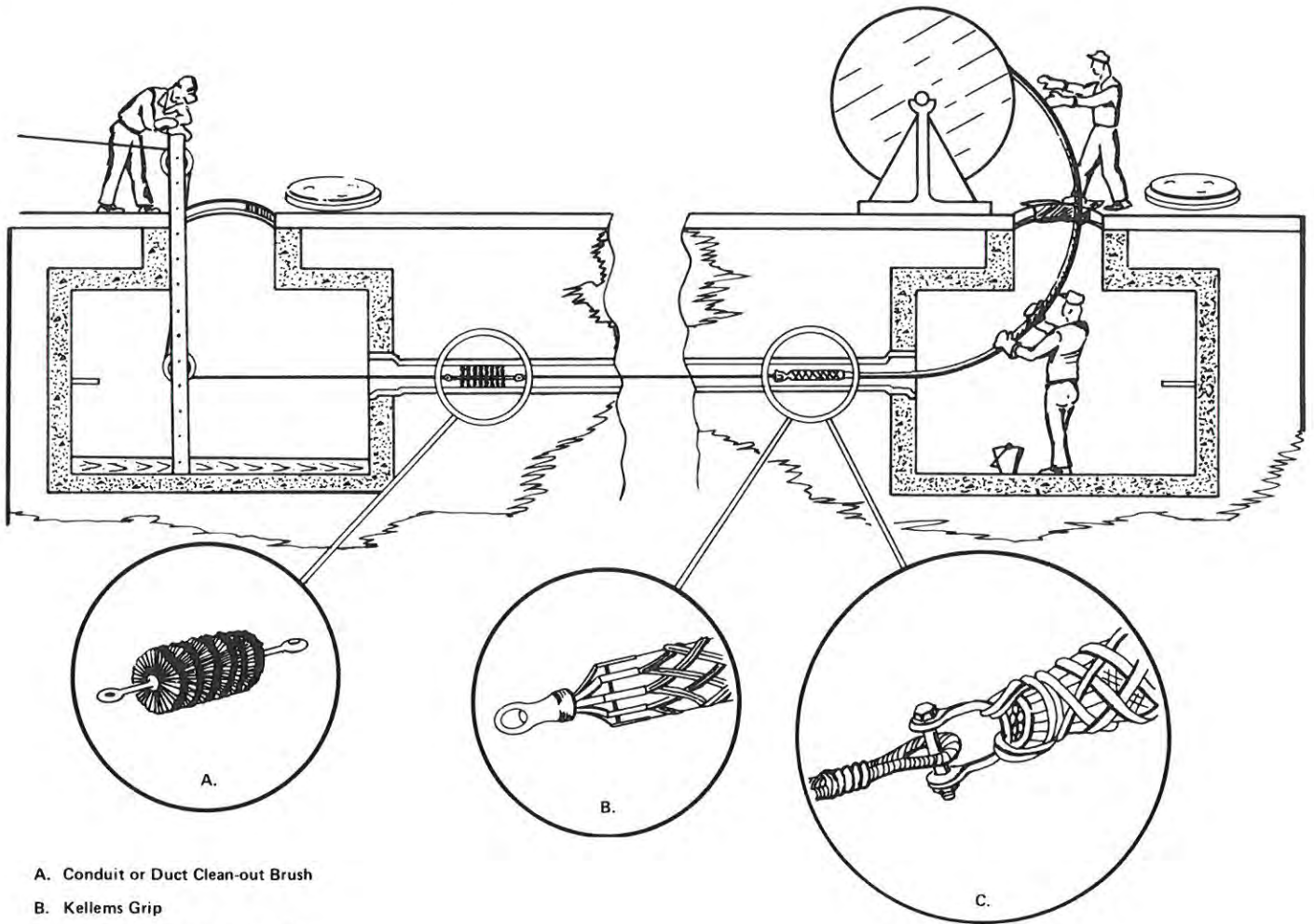
Fig. 11-21. Pulling cable in duct. Pulling cable between junction boxes of conduit installations is similar.
