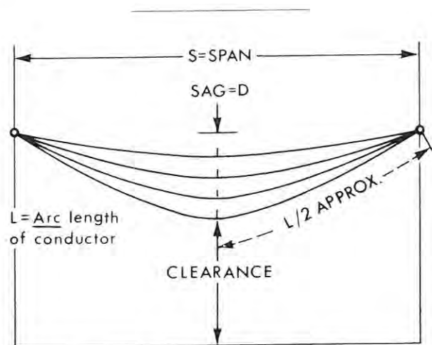
Fig. 5-1. Diagram showing family of sag curves. The sag is less with increase of conductor tension.
