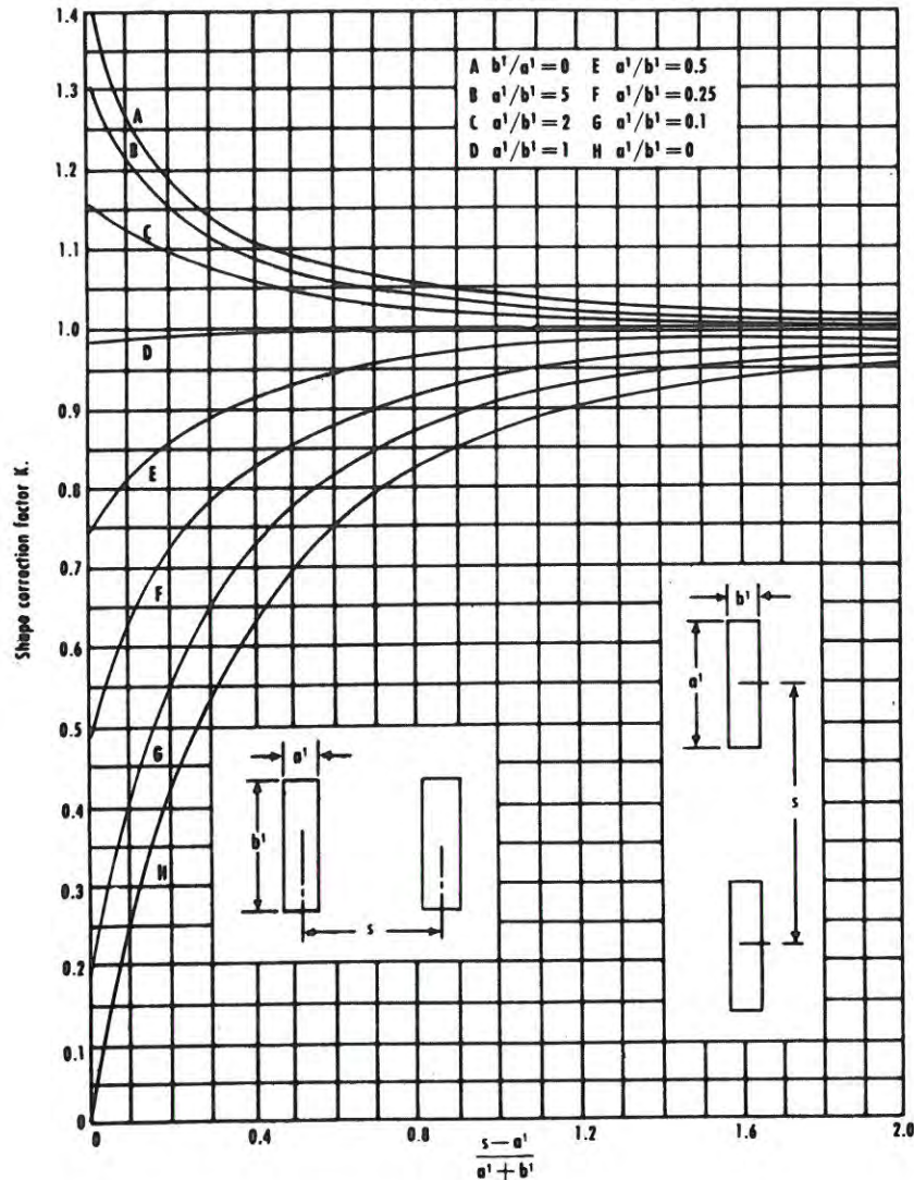
Fig. 13-12. Shape correction factor K for the calculation of electromagnetic force.
