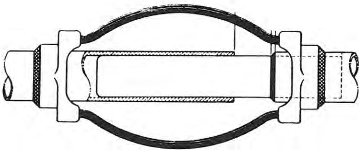
b. Welded Expansion Coupler Connector
