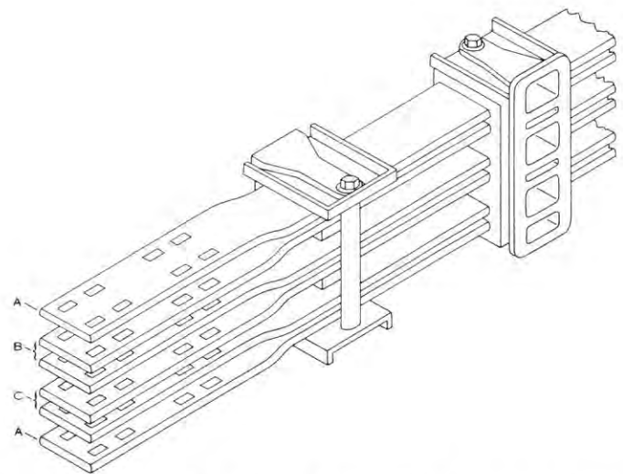
Fig. 13-28. Typical plug-in busway. The molded plastic plug-in blocks open alternately on opposite sides so connection can be made to any pair. The bars are immersion insulated between plug-in blocks and terminals. They are paired to reduce reactance AB BC CA. The arrangement shown is suitable for three-phase delta. By adding a neutral bar three-phase wye loads can be supplied. There are many varieties of plug-in busways for each of which advantages are claimed.
