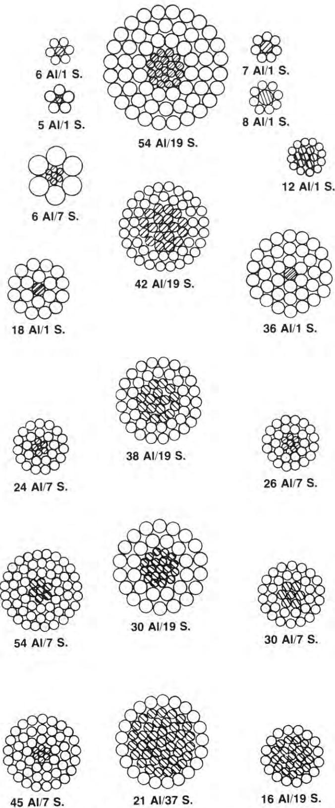
Fig. 3-4. Typical stranding arrangements of aluminum cable steel-reinforced (ACSR). The conductor size and ampacity for any arrangement depends on the size of the individual wires.
