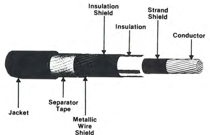
Fig. 10-13. Typical 5 kV to 35 kV shielded insulated primary cable.
