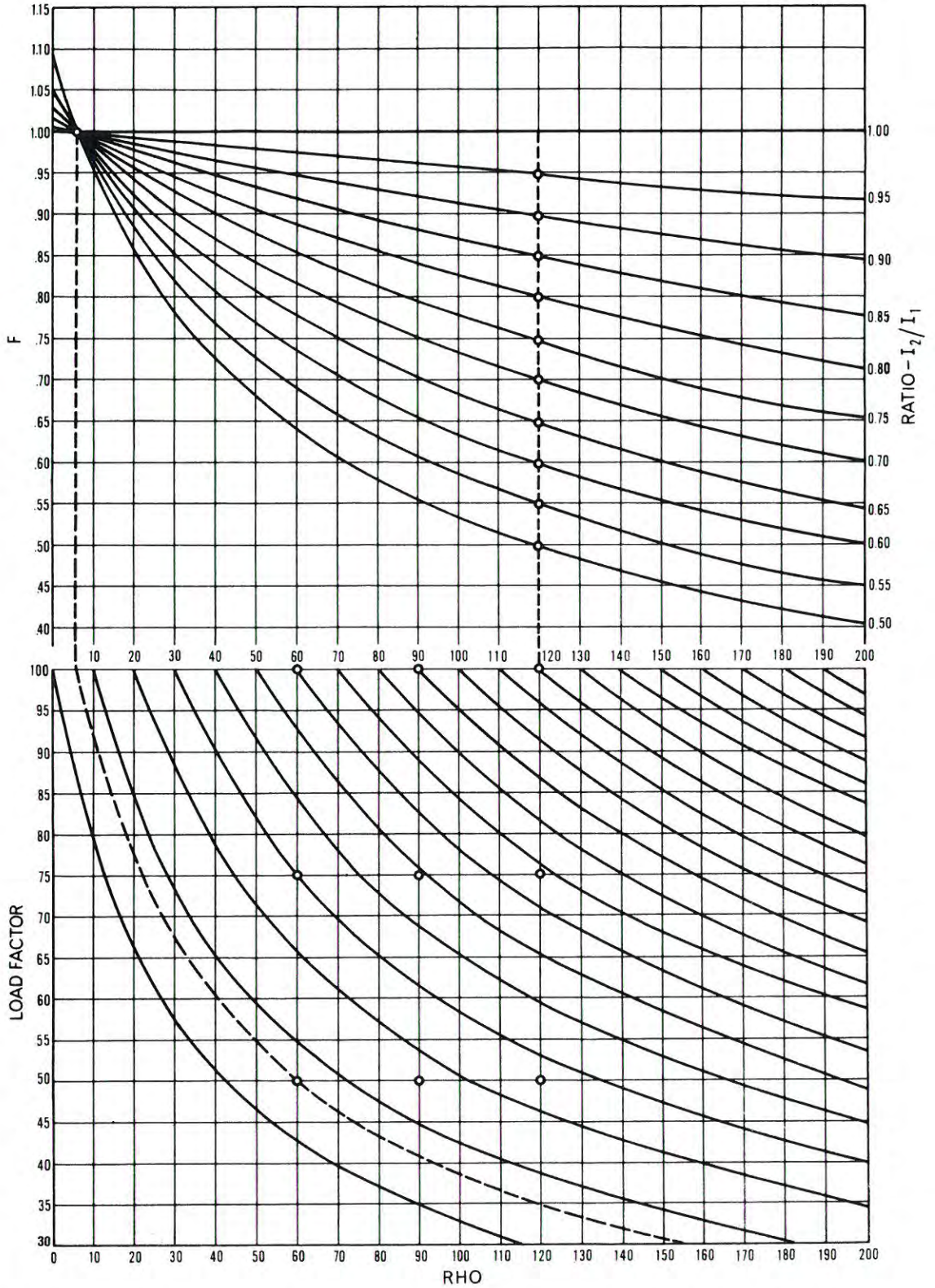
Fig. 9A-3. Interpolation chart for cables in a duct bank. I_1 = ampacity for RHO-90, 50 LF; I_2 = ampacity RHO-120, 100 LF; desired ampacity = F \times I_1 .
