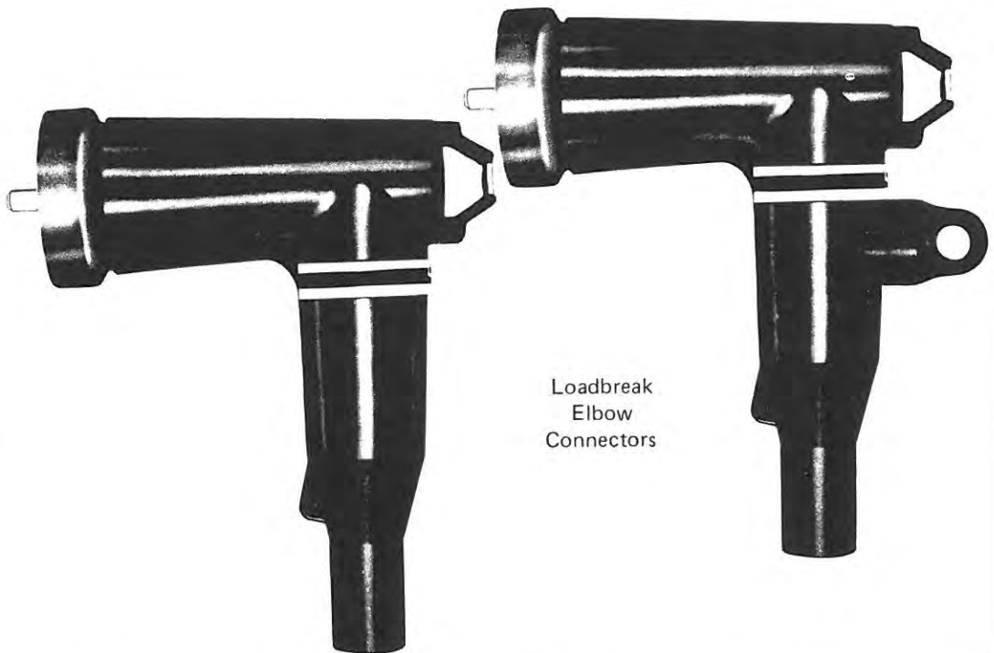
Fig. 11-26. Some typical primary voltage premolded splicing and terminating devices.
