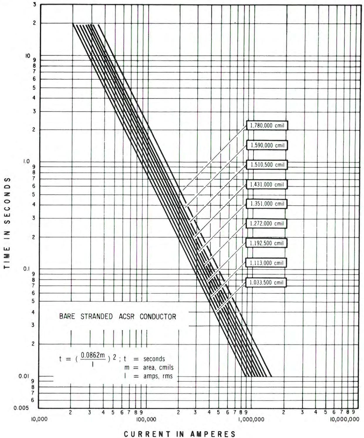
Fig. 6-2C. Maximum Fault-Current Operating Limit for Bare Stranded ACSR conductor. Upper temperature limit 645°C, ambient temperature 40°C.
