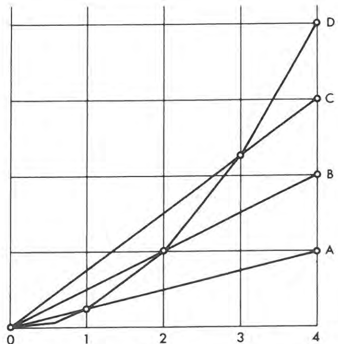
Fig. 5-9. Diagram for plotting points on a parabola.
