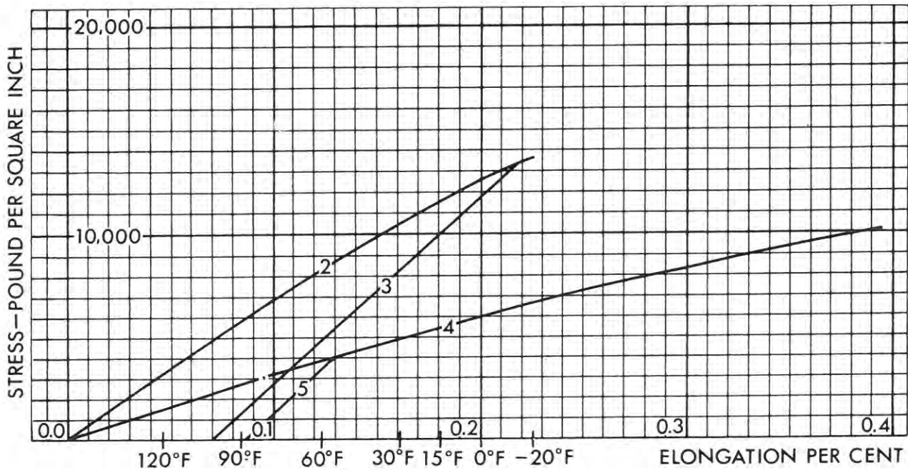
Fig. 5-10. Stress-strain curves.
