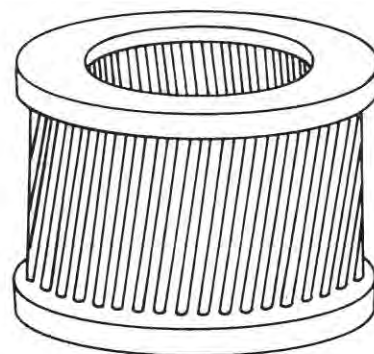
Fig. 16-3. Iron surrounding the cast-aluminum squirrel cage has been removed to reveal construction.
