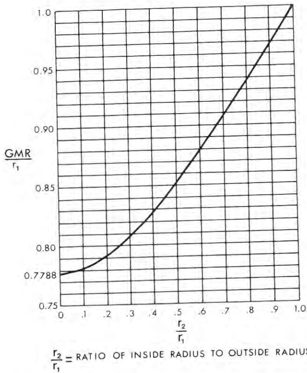
Fig. 3-10. GMR of annular rings. L. F. Woodruff, "Electric Power Transmission and Distribution," 1938.
