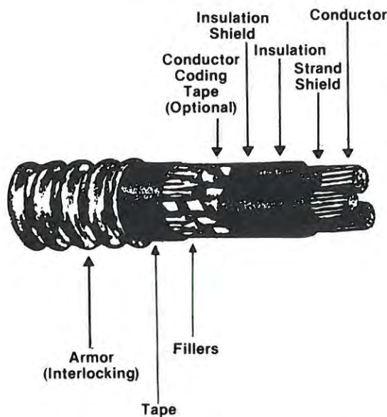
Fig. 10-16. Three-conductor shielded cable 5 kV to 15 kV with interlocked or impervious corrugated steel or aluminum armor.
