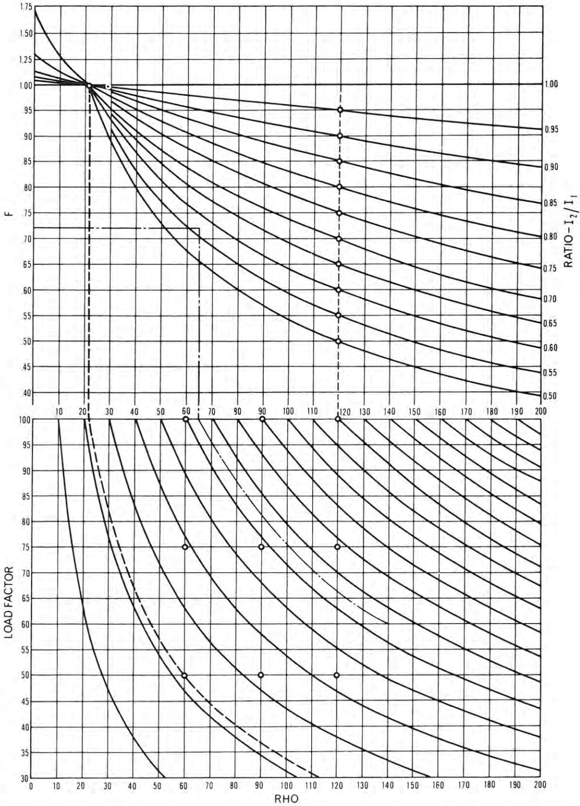
Fig. 9A-4. Interpolation chart for pipe-type and directly buried cables I_1 = \text{ampacity for RHO-60, 50 LF} ; I_2 = \text{ampacity for RHO-120, 100 LF} ; desired ampacity = F \times I_1 .
