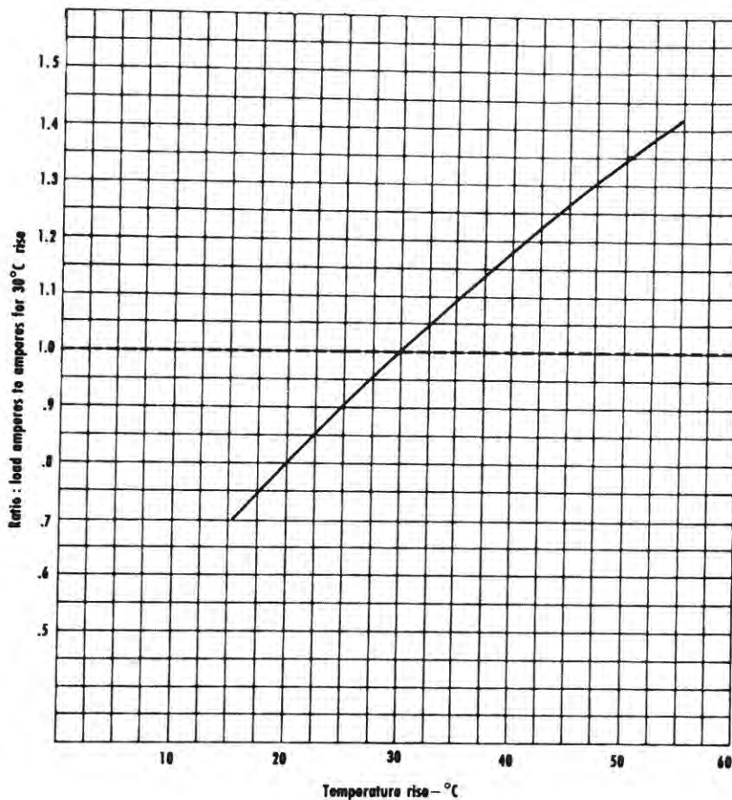
Fig. 13-11. Temperature rise vs. load ratio curve for aluminum bus conductors. Note: Based on calculations for dc current using formulas from Chapter 9, "Heat Transfer" of Electrical Coils and Conductors , 1945 McGraw-Hill Book Co. Checks approximately formula by Fugill. (See Eq. 13-4, page 13-22).
