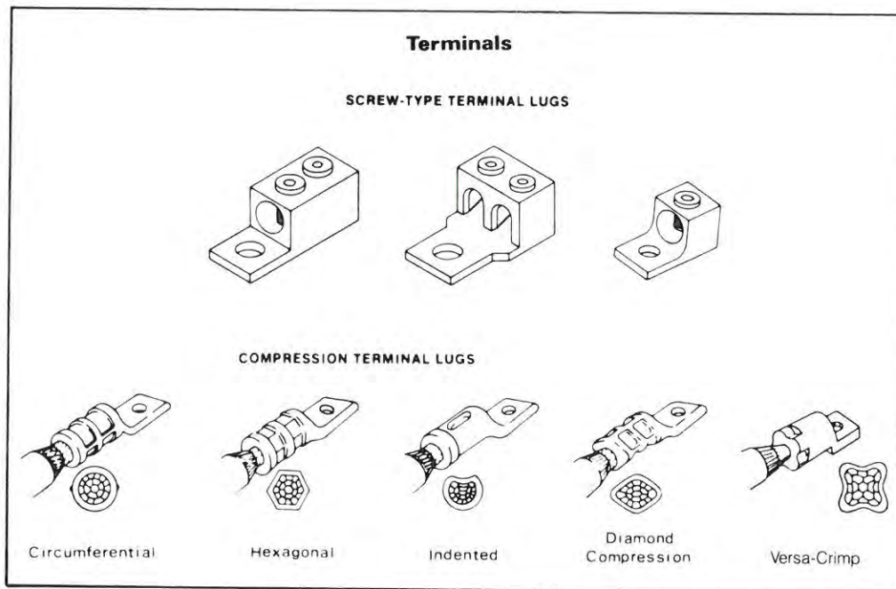
Fig. 11-2. Typical plated aluminum terminal lugs come in variety of styles.
