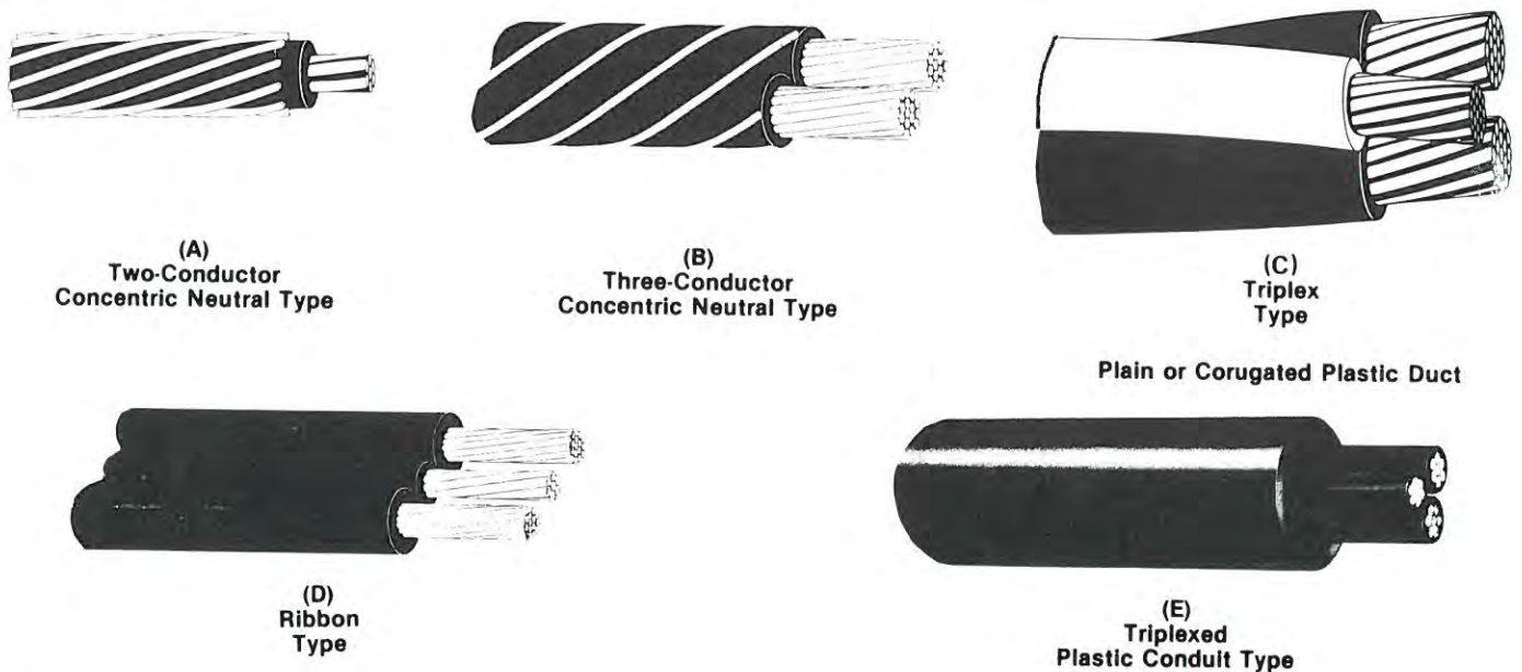
Fig. 10-9. Typical 600-volt cables for direct burial.
