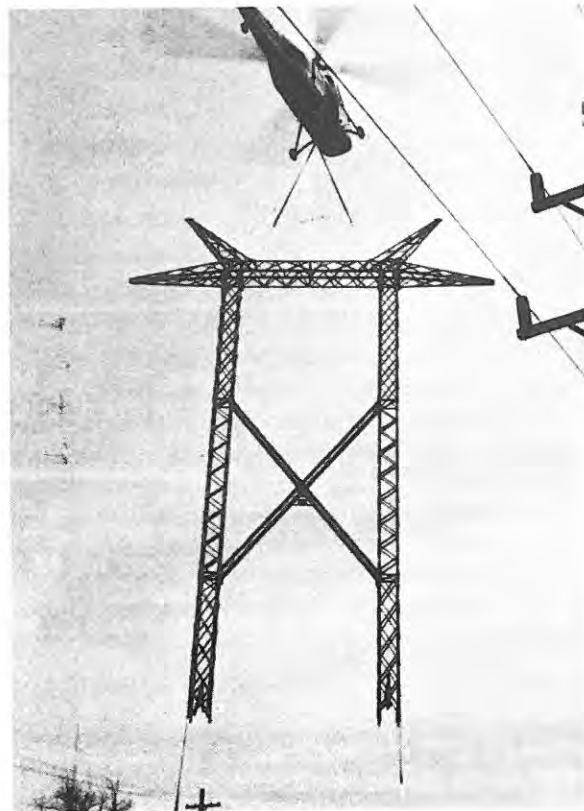
Fig. 18-8. Helicopter leaving assembly yard with "H" frame on Public Service Company of Indiana 345 kV line.
