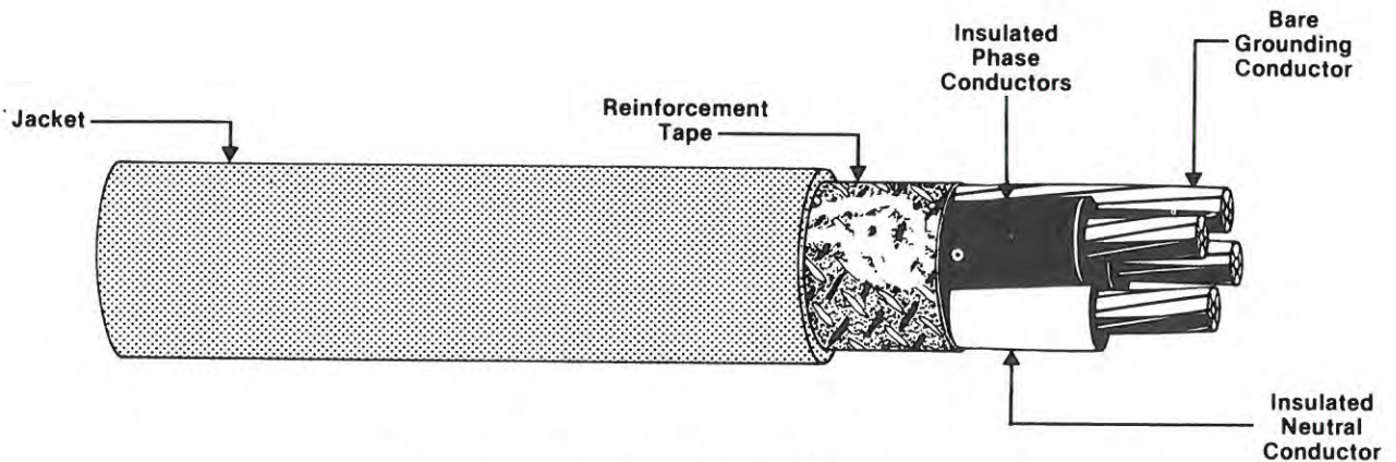
Fig. 10-5. Typical type SE-style SER cable.
