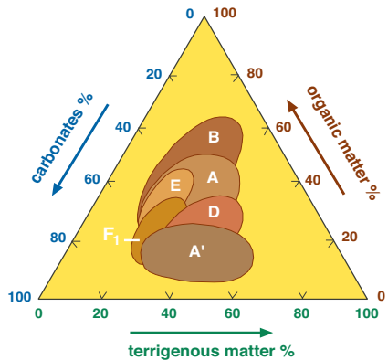
Triangular plot of main constituents in kukersite oil shale, Estonia deposit (H. Bauert ja V. Kattai, 1997, after Fig. 212)
