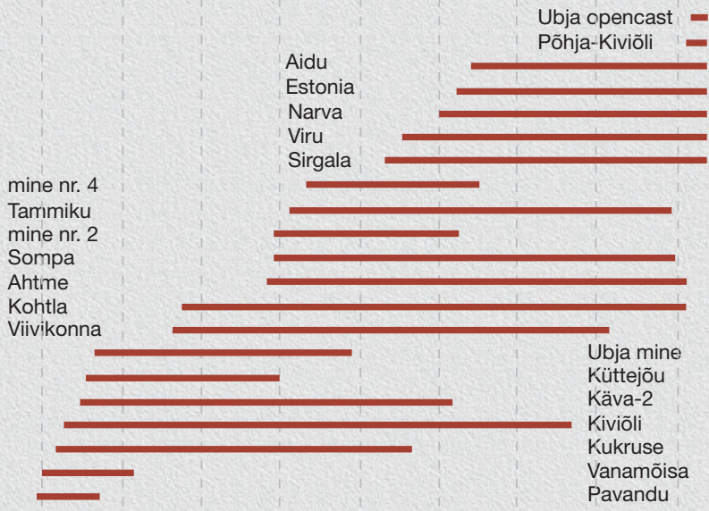
Oil shale mining and utilization in Estonia with bargraphs showing life-span of oil shale mines and opencasts (V. Kattai, 2003, after Fig. 5.4)
