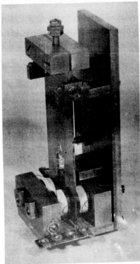
FIGURE 17 ANGULAR ACCELEROMETER UNDER CONSIDERATION FOR USE IN MAIN CONTROL SERVO SYSTEM
