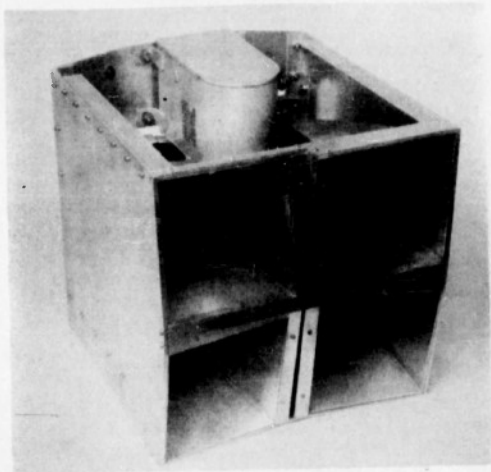
FIGURE 6 - FRONT VIEW OF HORNS OF ANTENNA SYSTEM FOR KINGFISHER
