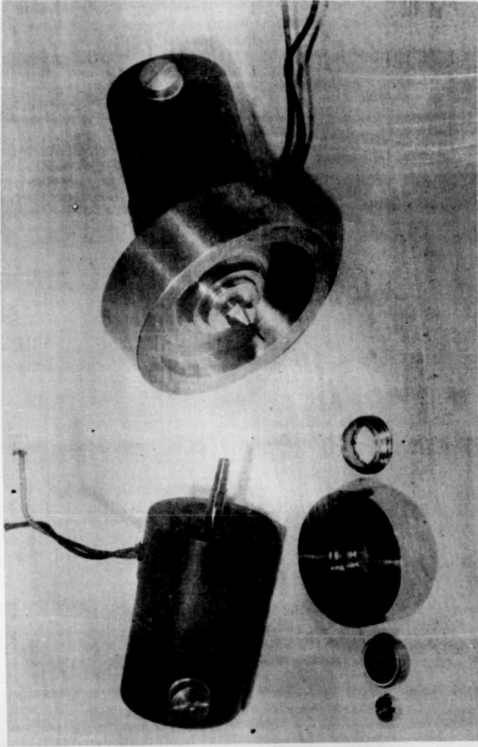
FIGURE 13 TWO GYROSCOPES DEVELOPED FOR CONSIDERATION AS THE FREE GYRO IN ANTENNA STABILIZING SYSTEM
