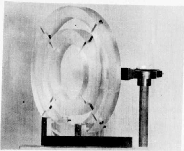
FIGURE 9 - FRESNEL ZONE PLATE LENS (A six-inch scale is at the bottom of the lens)
