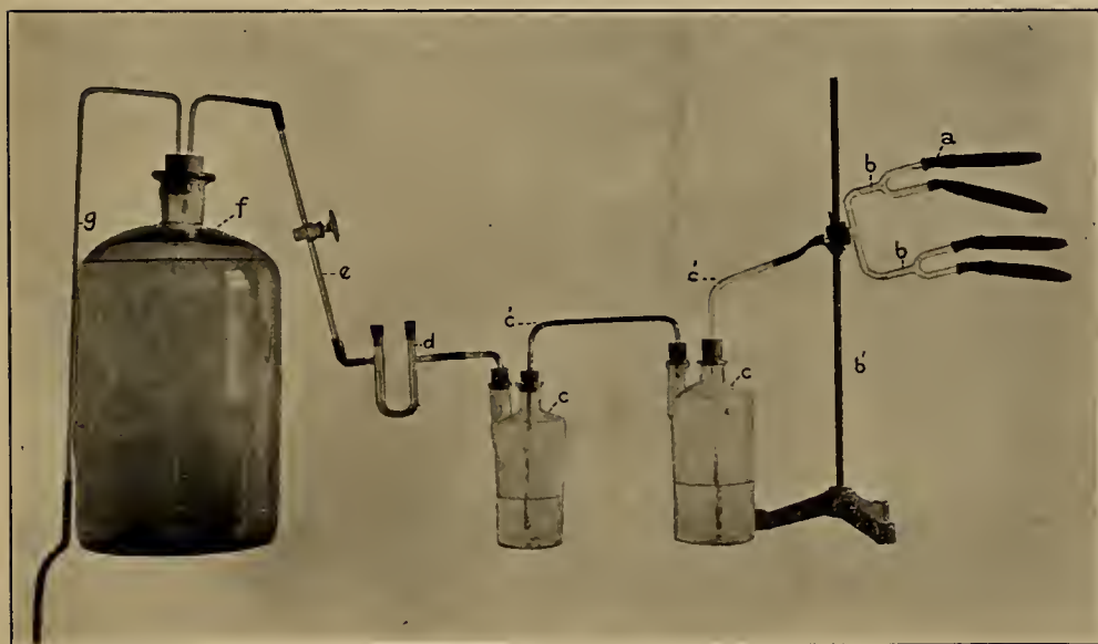
Fig. 2. Apparatus used for testing cigars.
