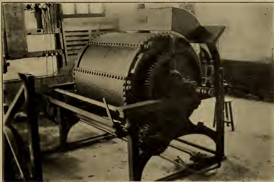
Fig. 2. A revolving steam drum.
