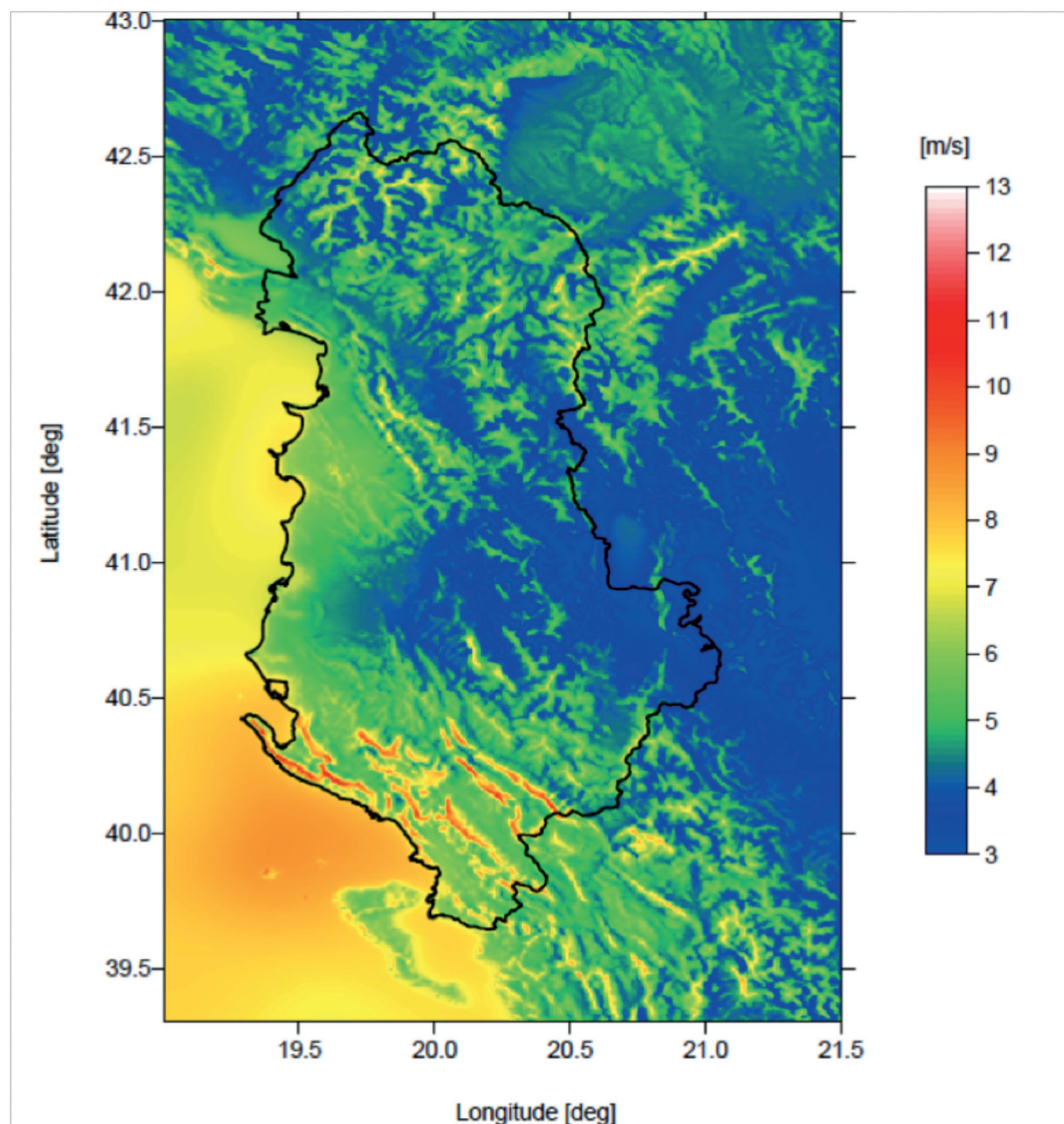
Figure 3: Average Wind Speed at 50 m a.g.l. over the Albanian Territory
